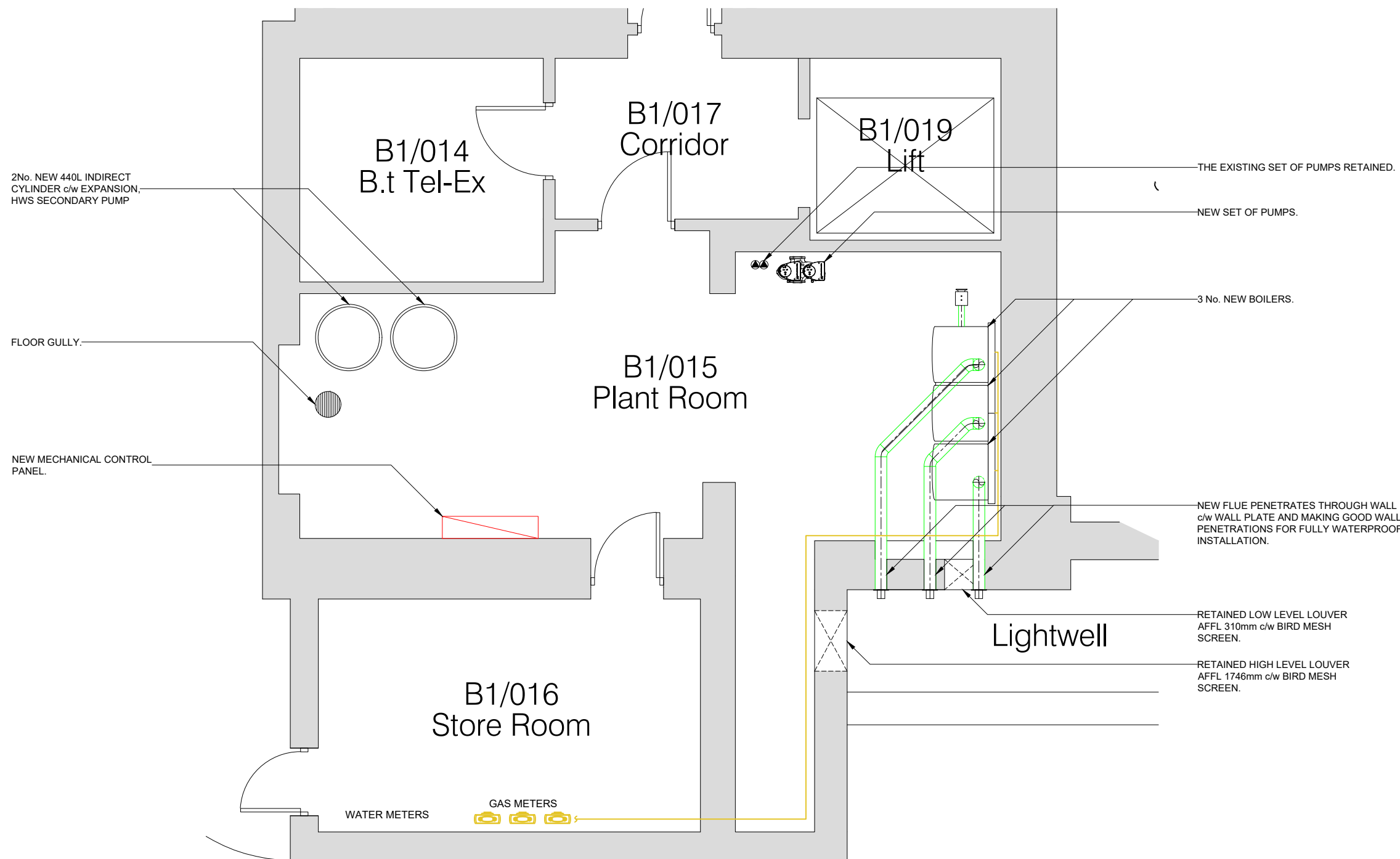
BASEMENT PLAN
