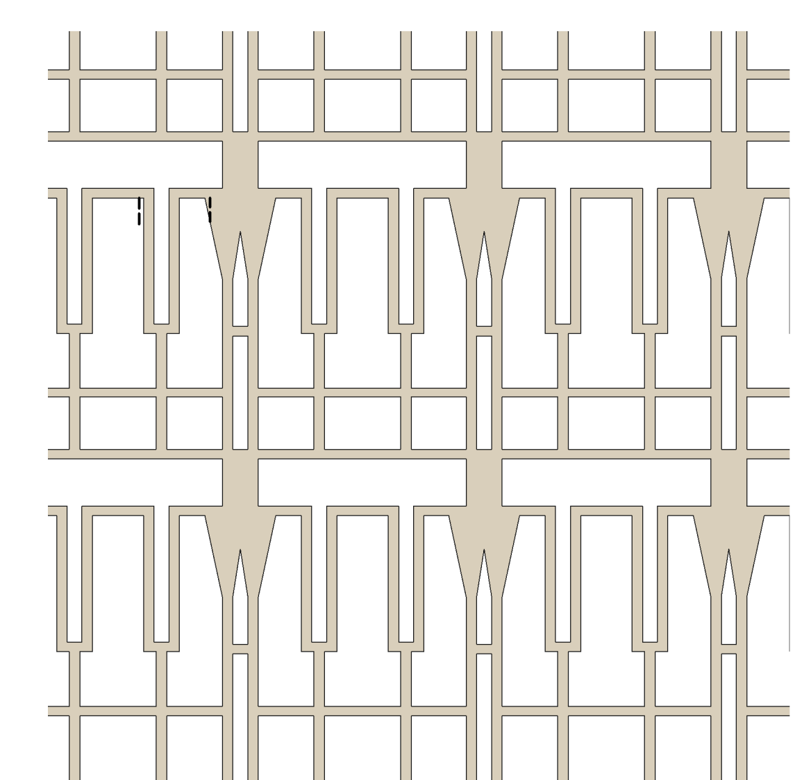
3 Elevation - Detail of grillage pattern 4 1 : 5
