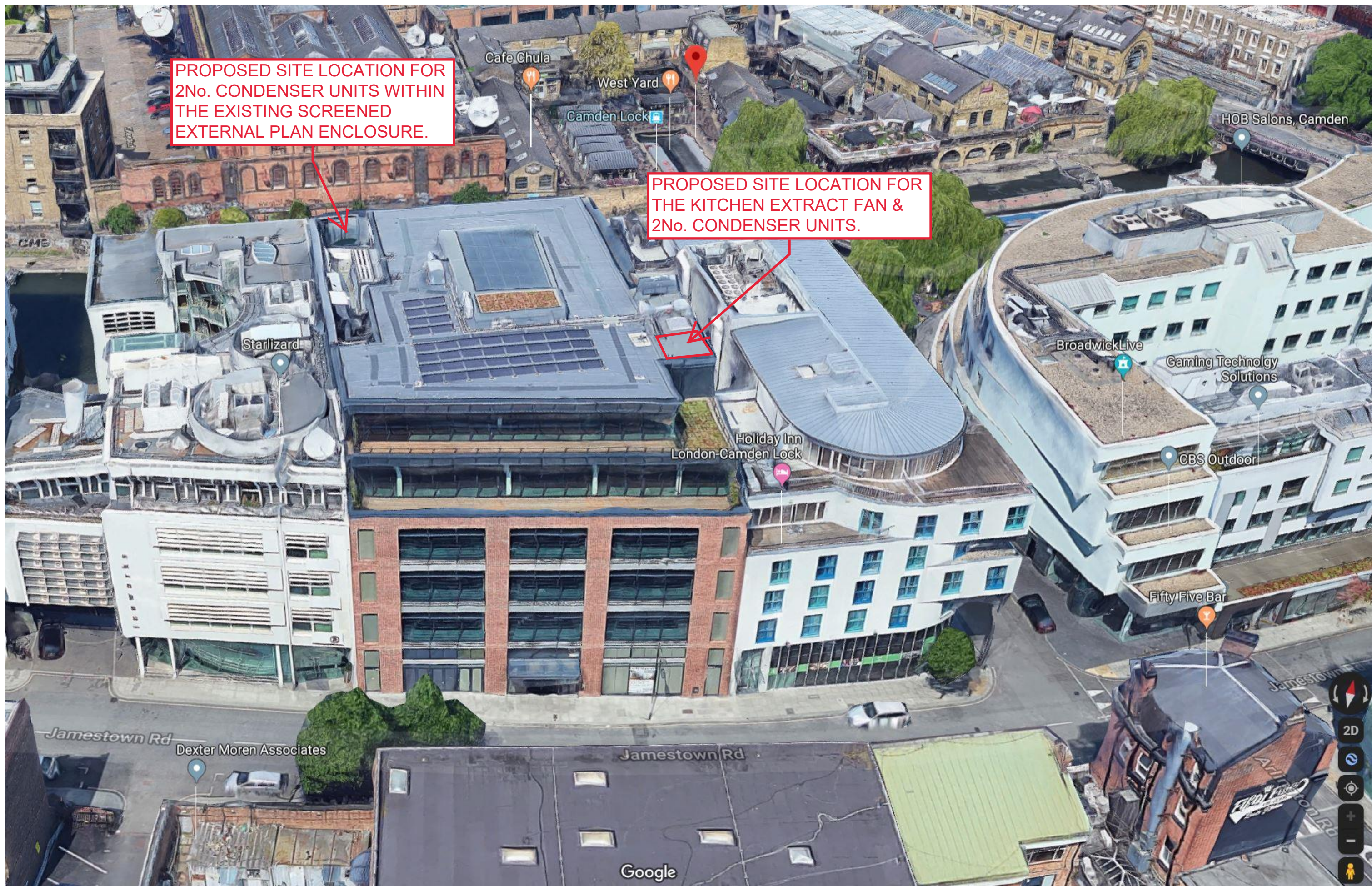
SSP - Jamestown Wharf: Planning Application Site Plan (Roof Space for Extract Fan, Duct Work & External Condensers)
