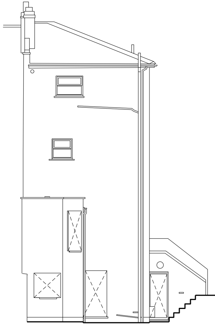
ELEVATION 1 (FROM CAMDEN PARK RD) (lower ground and ground floor windows and door shown with existing security hoarding)
