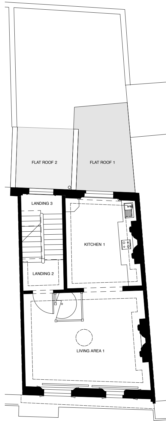
3 existing first floor plan
