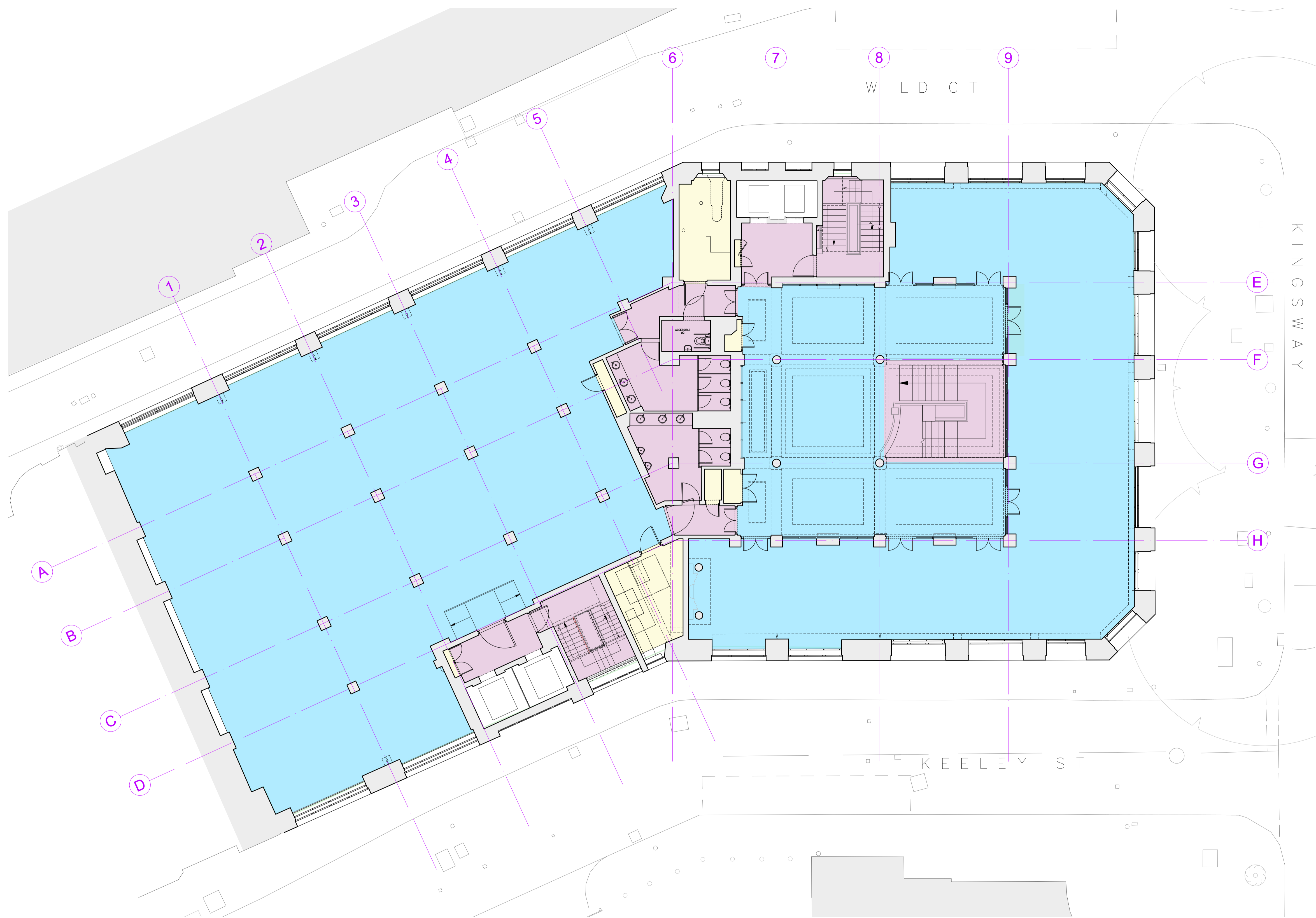
01 Existing First Floor Plan 1:100@A1, 1:200@A3
