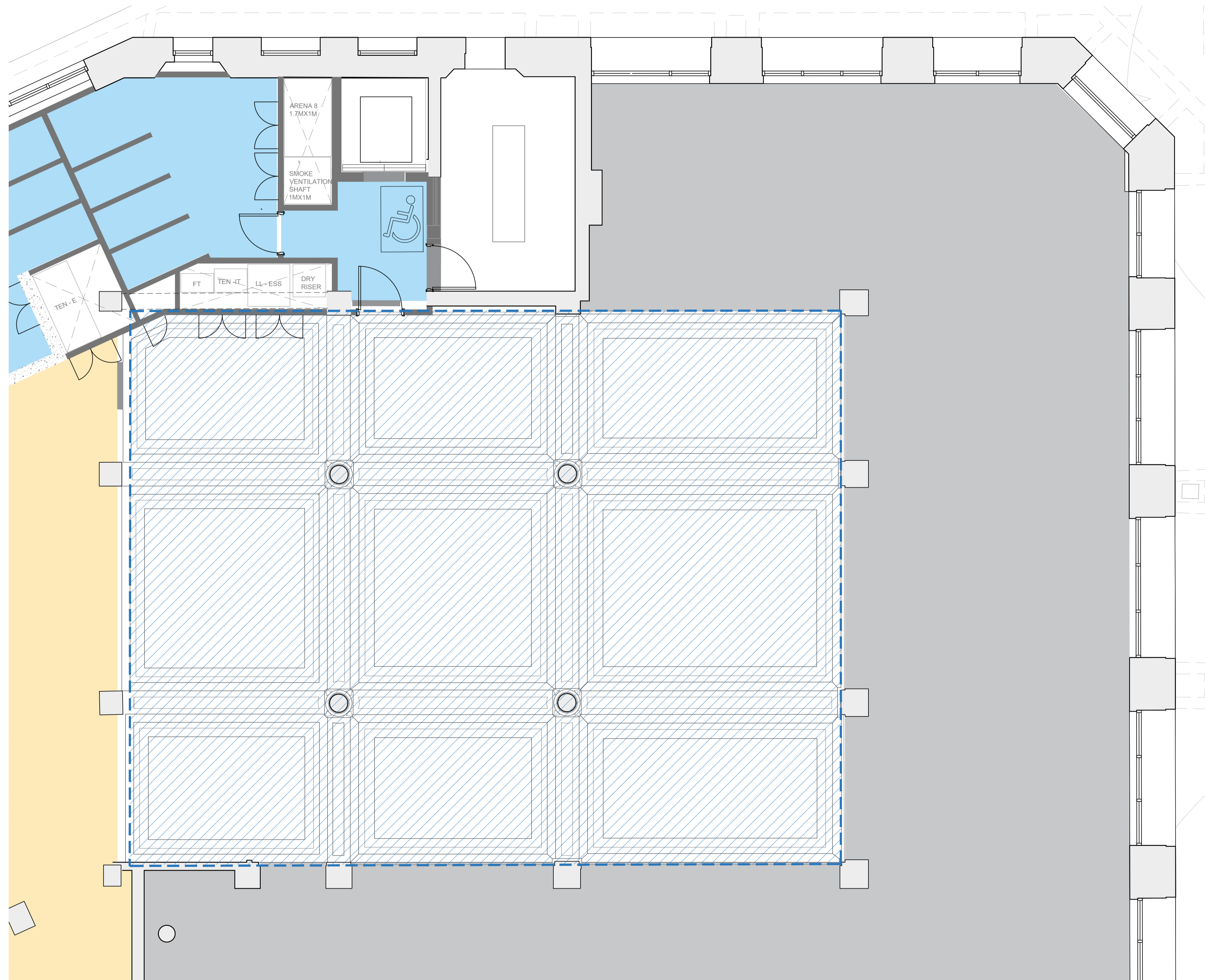
01 Proposed First Floor Ceiling Plan Detail 20.203 1:50@A1, 1:100@A3
