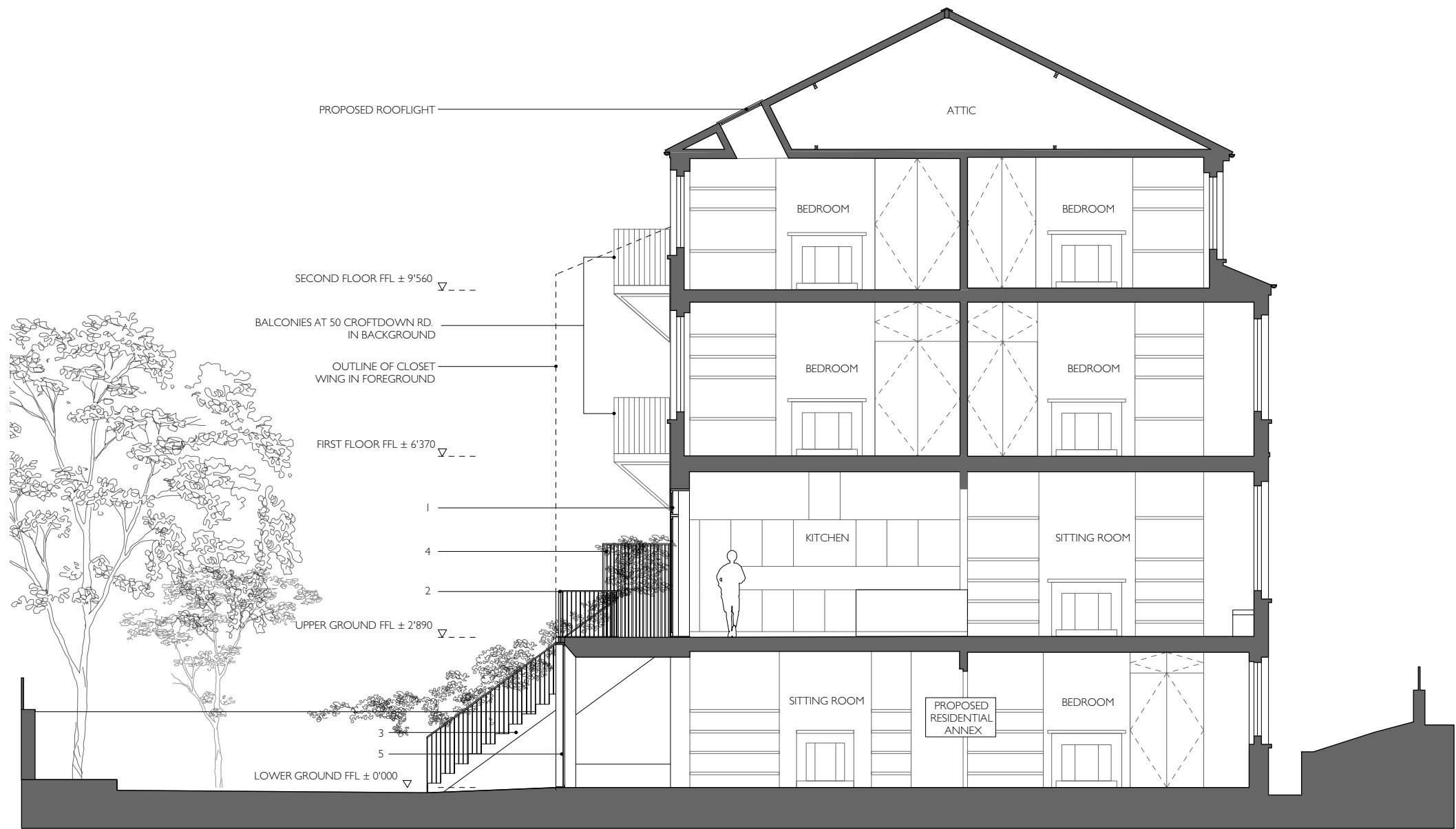
01 PROPOSED SECTION AA
