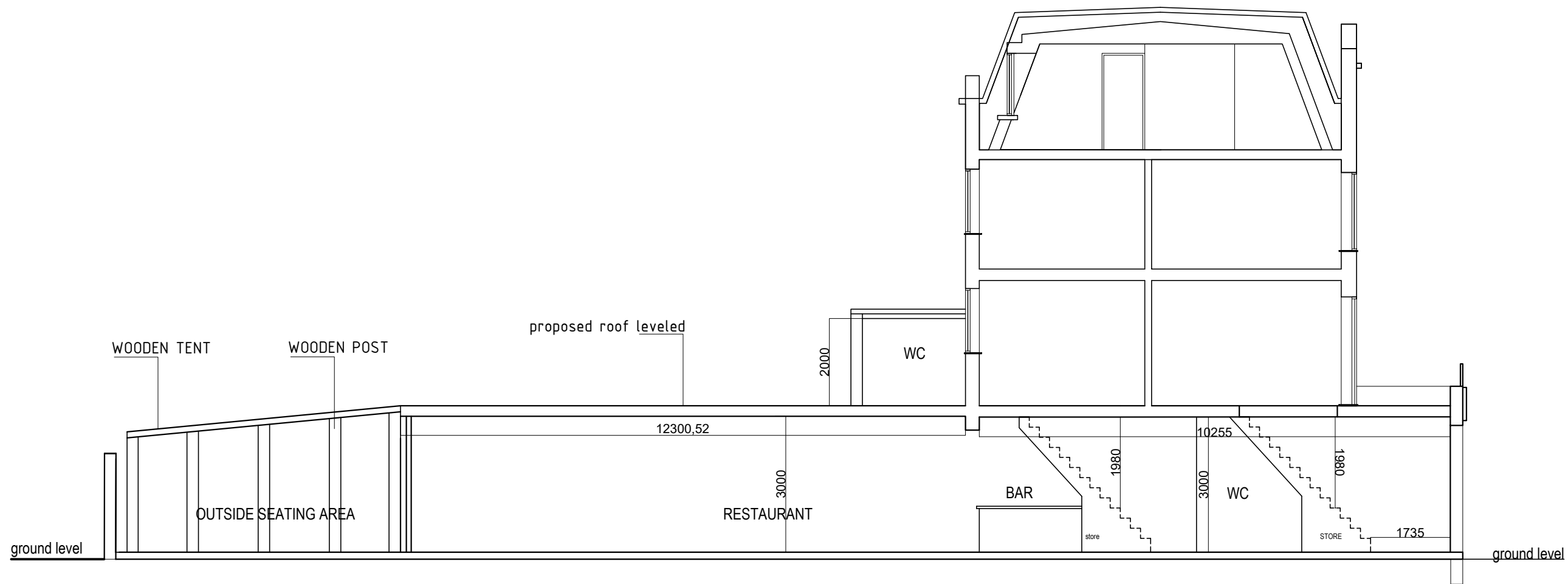
PROPOSED A-A SECTION SCALE: 1/100
