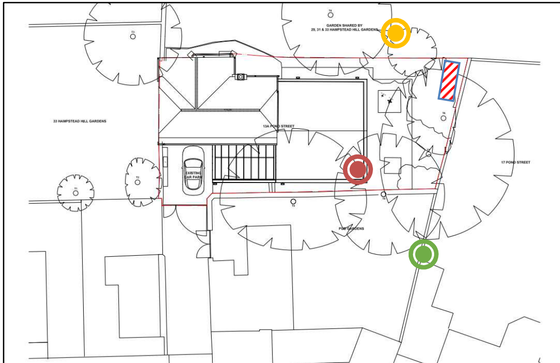
Figure 2.2 Site measurement position, identified receiver and proposed plant unit installation (Drawing Source: Gianni Botsford Architects)
