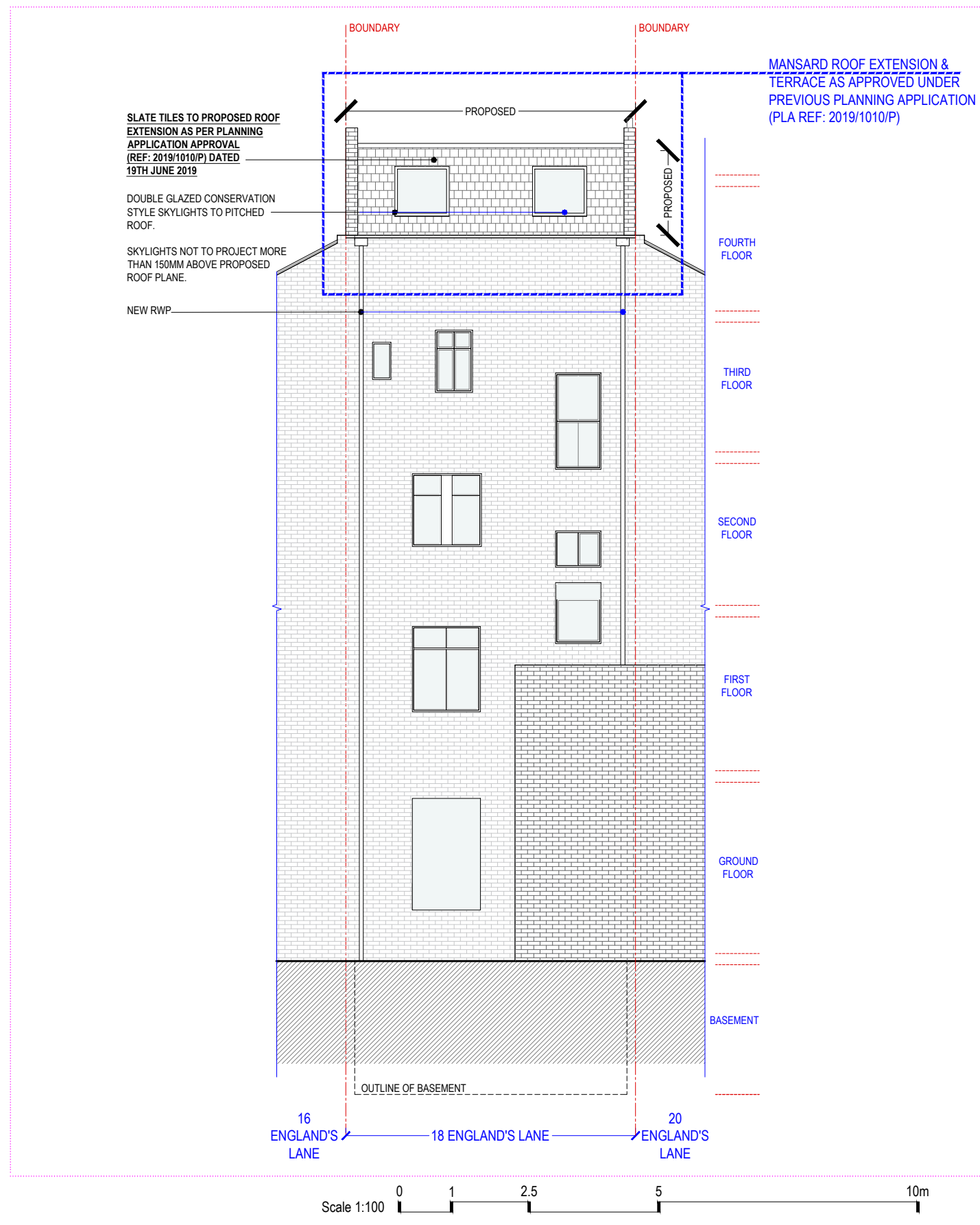
[01] PROPOSED REAR ELEVATION @1:100
