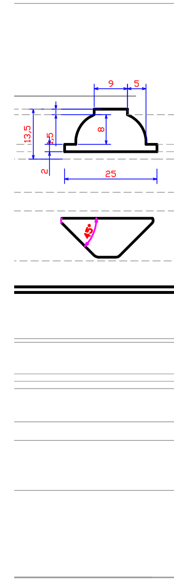
5 Glazing Bar Scale 1:1
