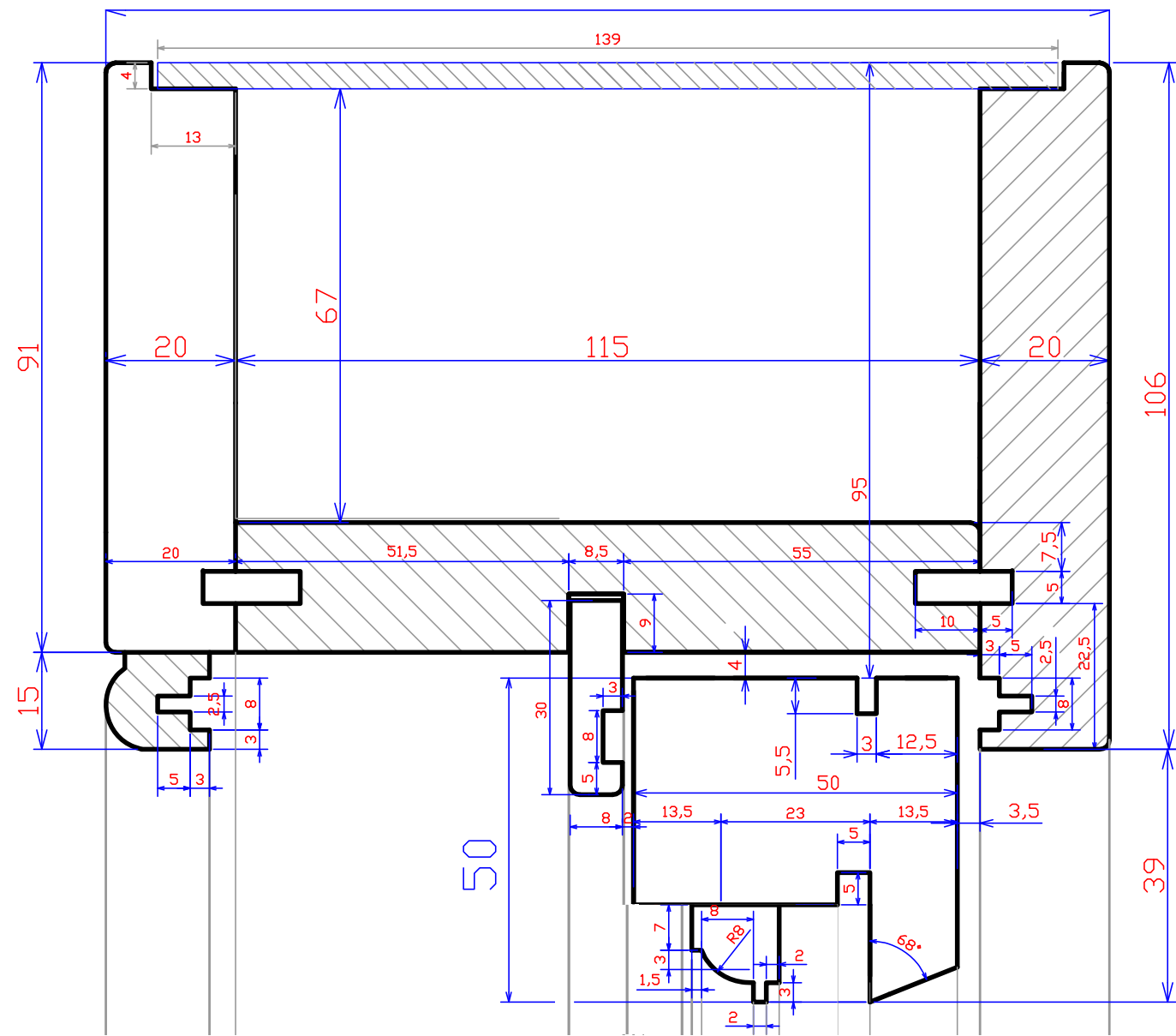
3 Head Scale 1:1
