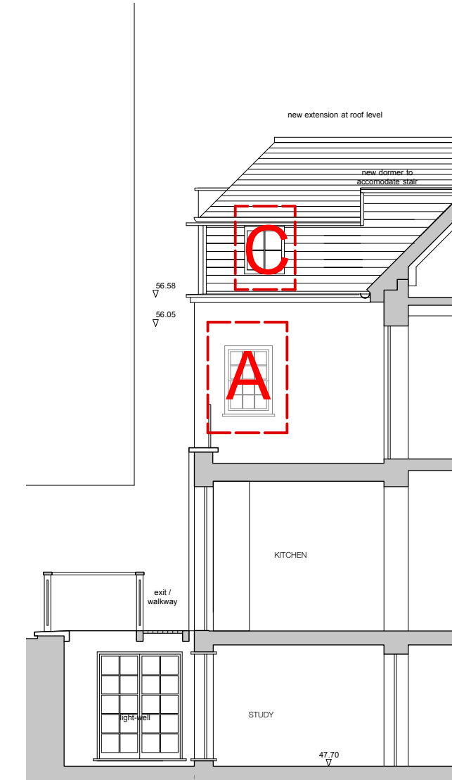
K2 Key: Side Elevation Scale 1:100
