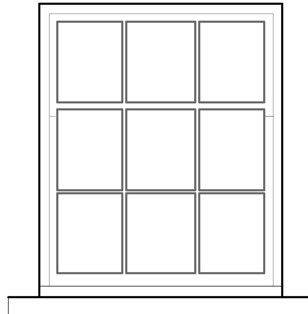
B Sash Window; Type B 1:10
