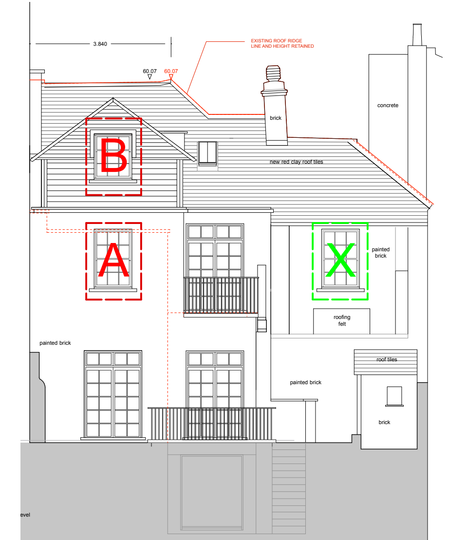
K1 Key: Rear Elevation Scale 1:100
