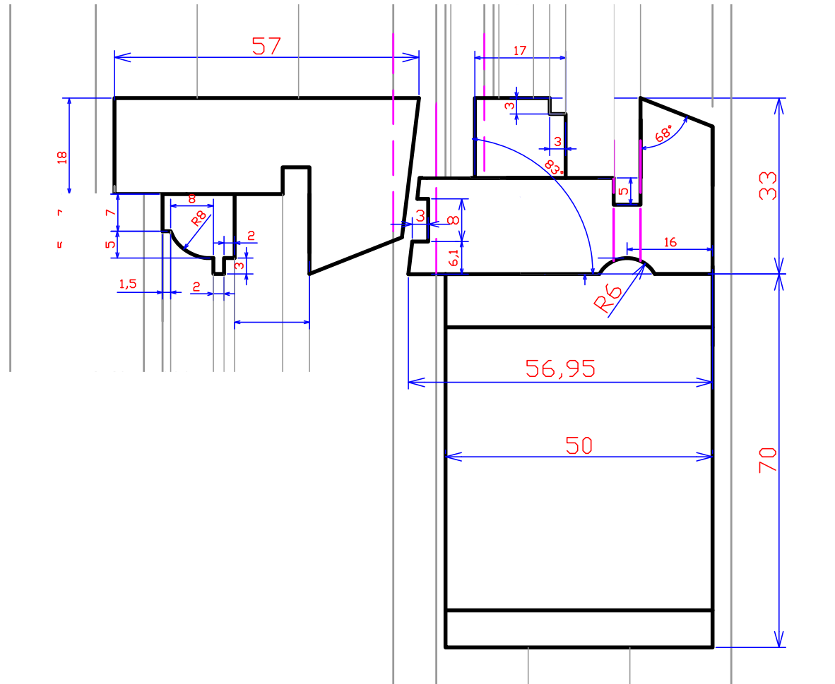
2 Meeting Rails Scale 1:1
