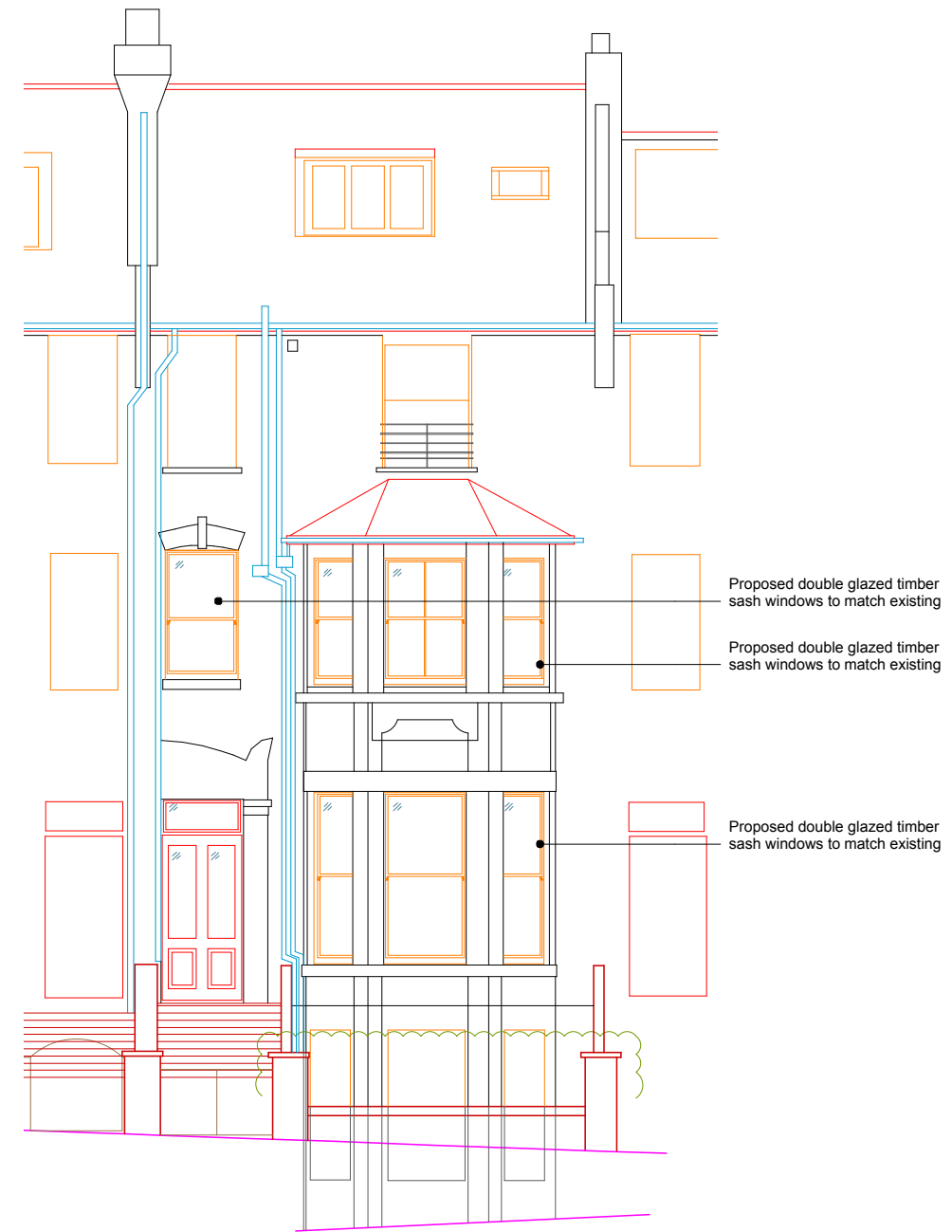
Proposed front facade
