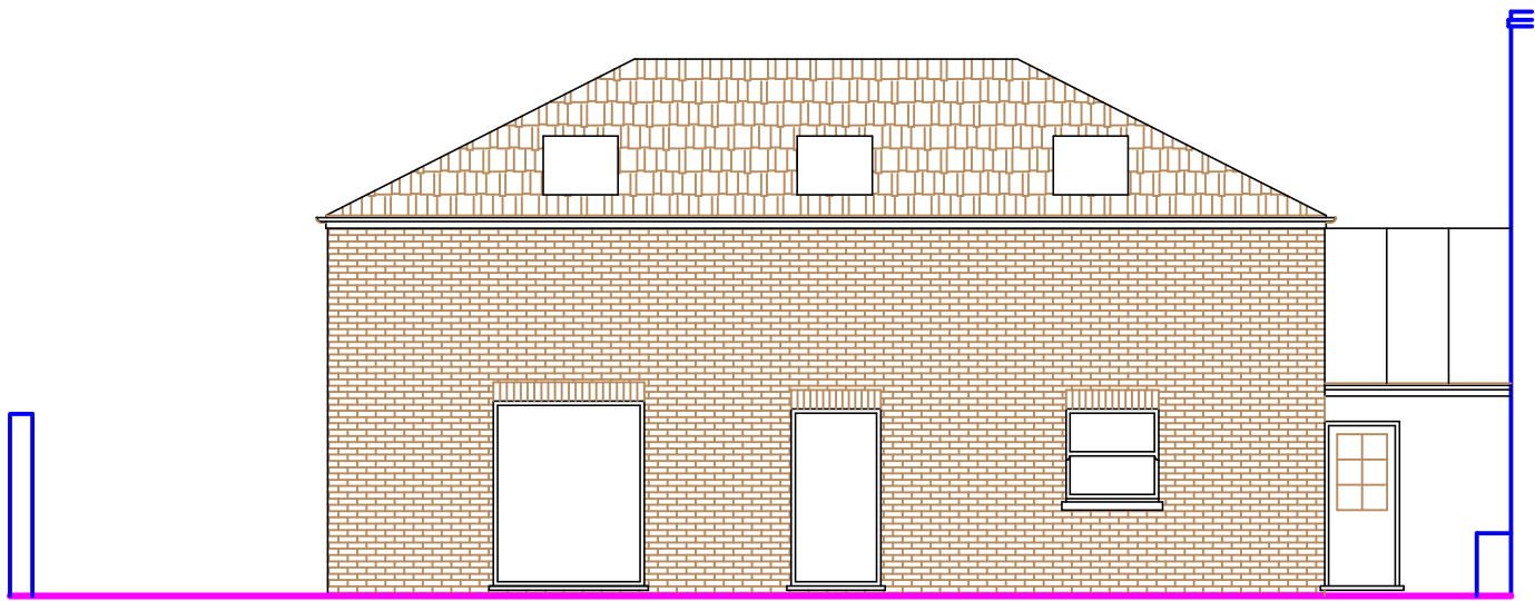
SIDE ELEVATION -as existing-
