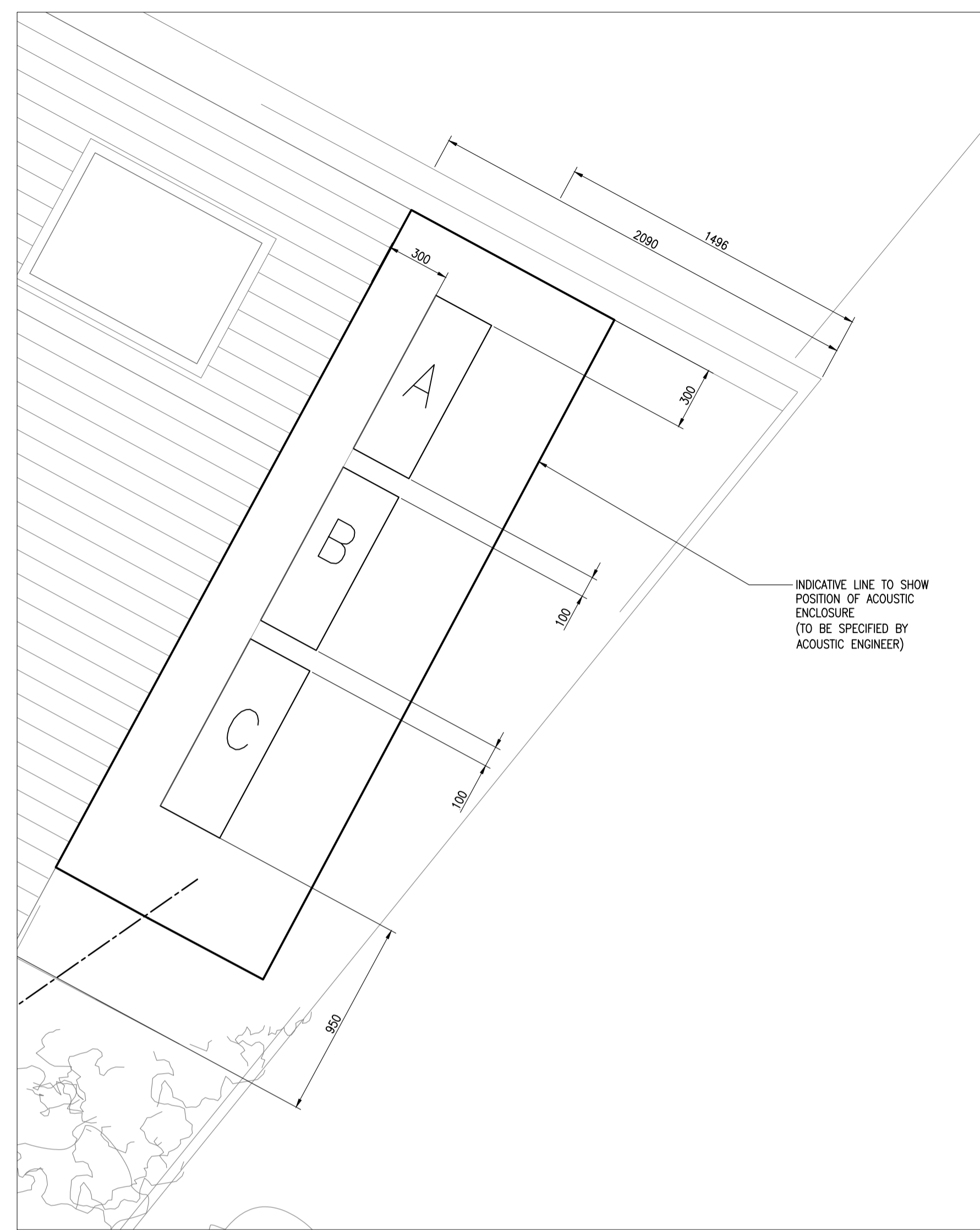
DETAIL A 1:20
