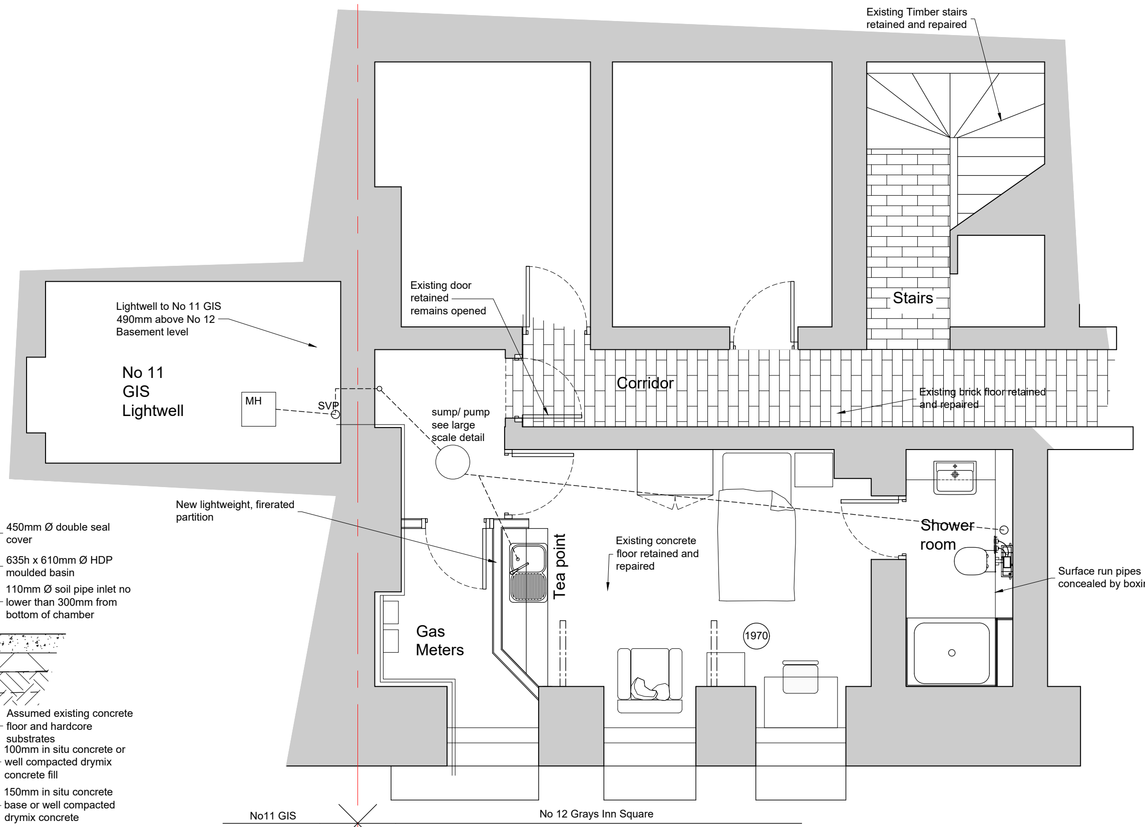
12 GIS Basement Plan as proposed
