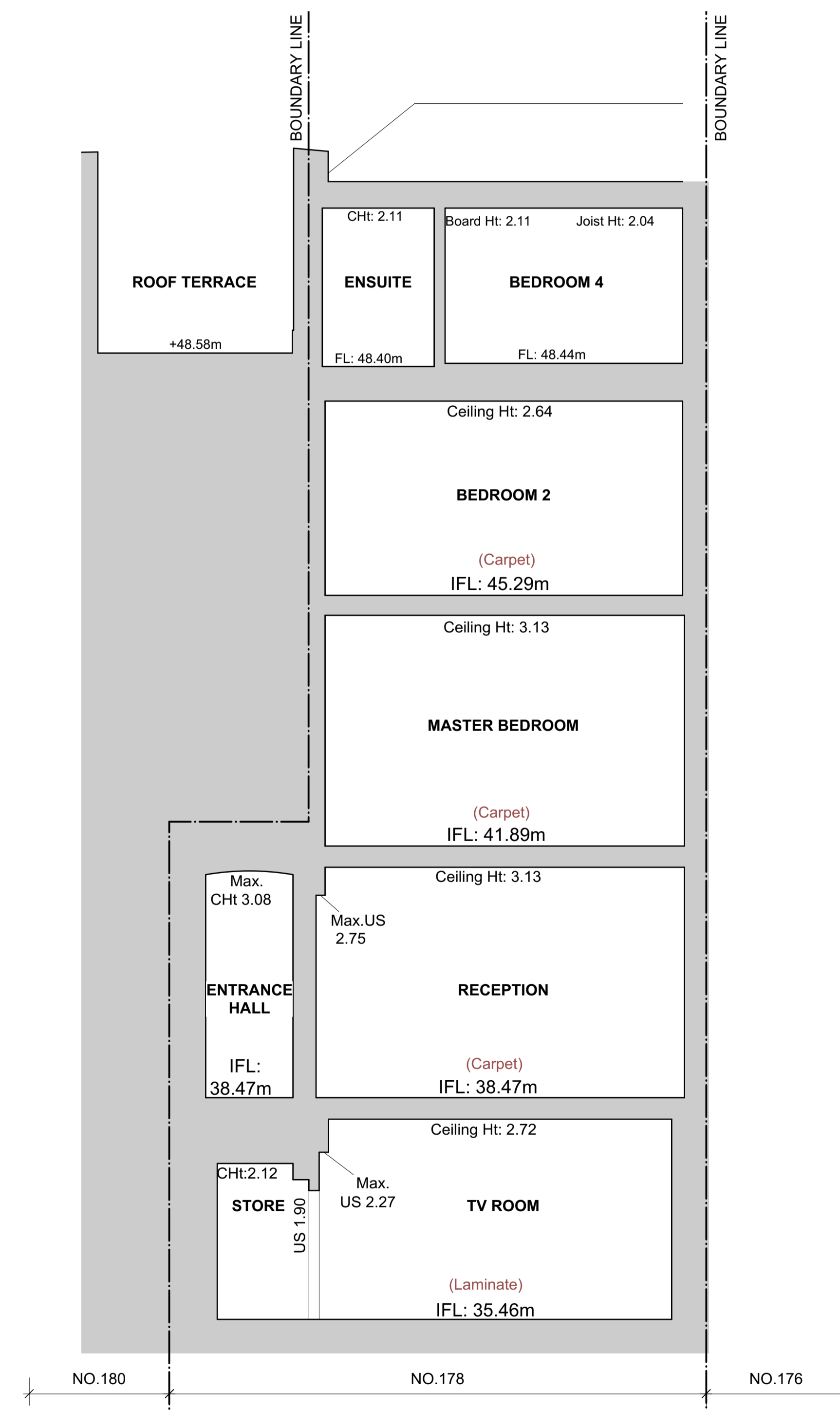
2 Existing Section B 1:50-A1/1:100-A3
