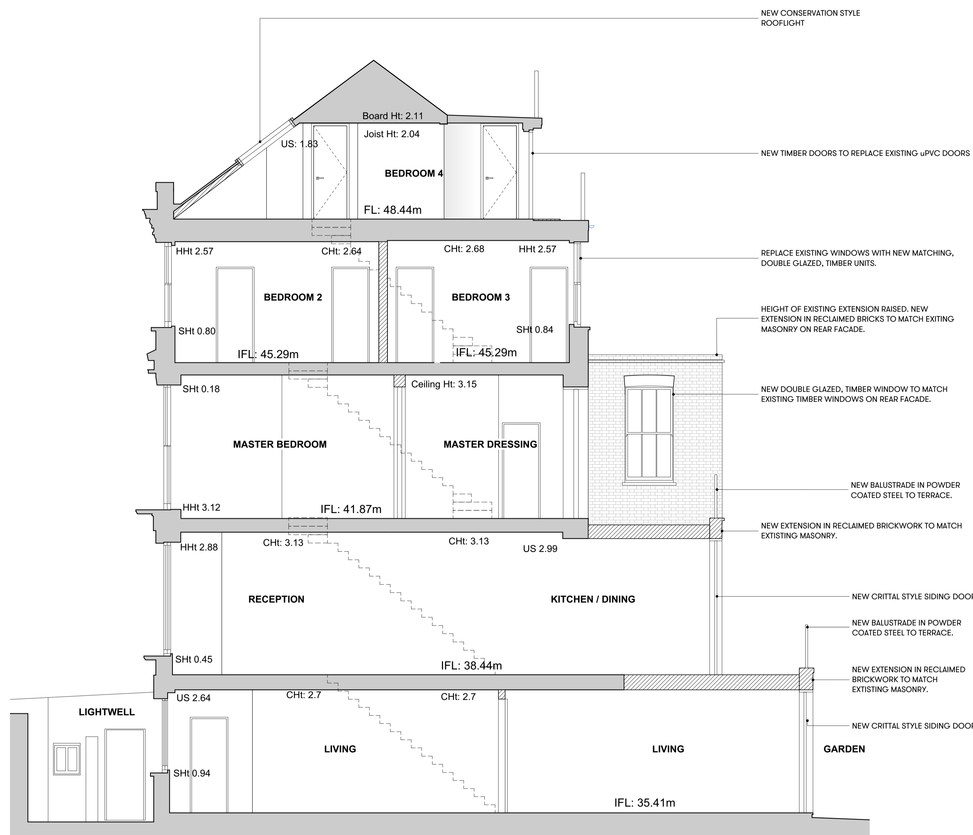
1 Proposed Section A Scale: 1:50-A1 / 1:100-A3
