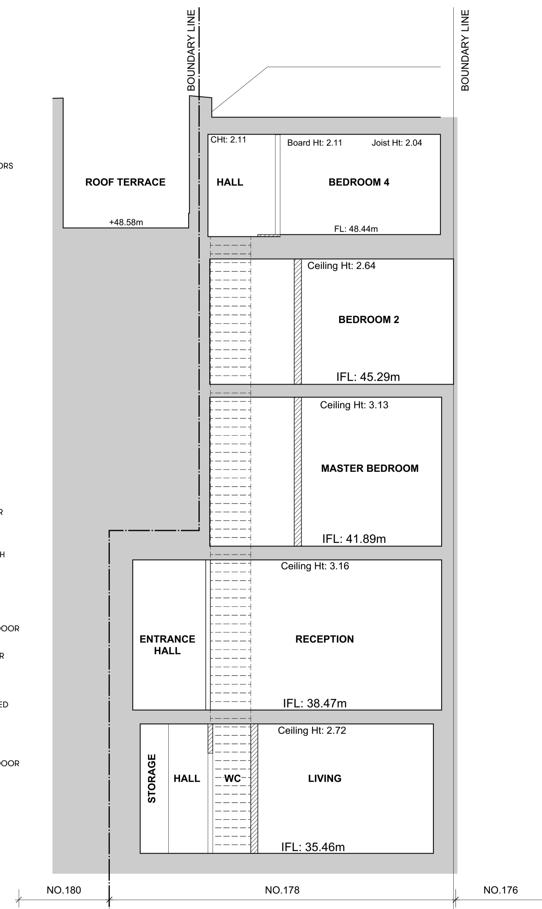
2 Proposed Section B Scale: 1:50-A1 / 1:100-A3
