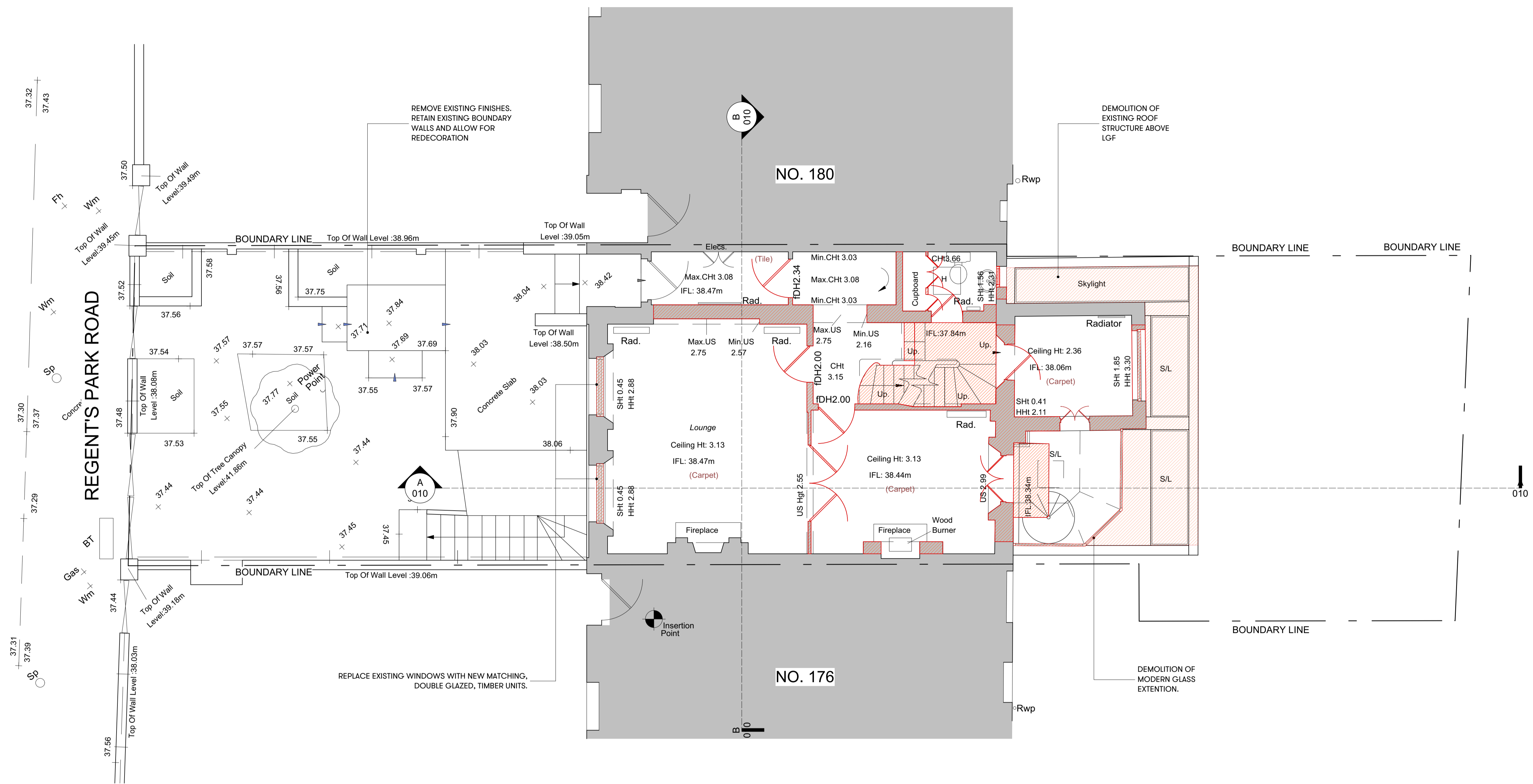
1 Proposed GF Demolition Plan Scale: 1:50-A1 / 1:100-A3
