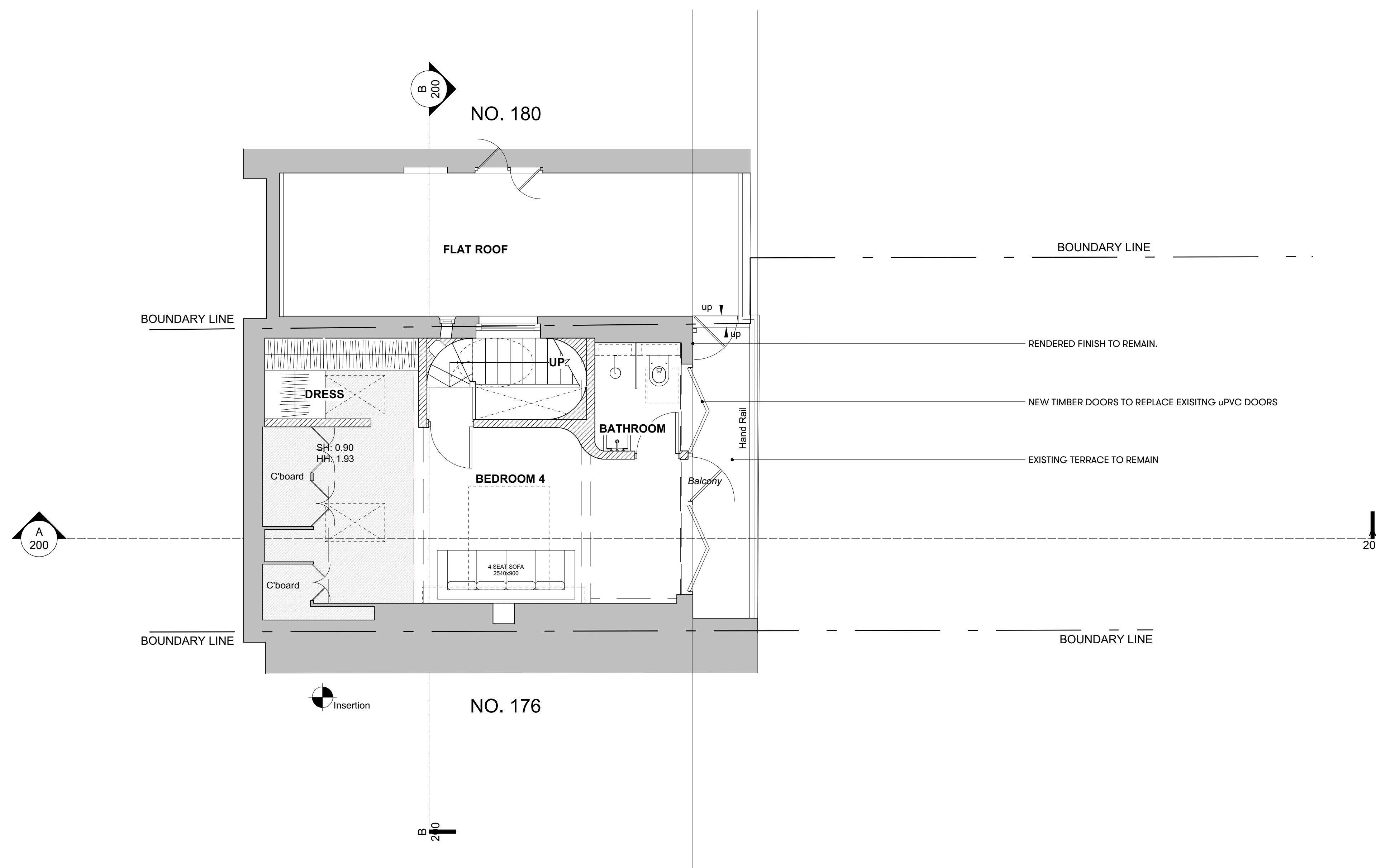
1 Proposed 3F Plan Scale: 1:50-A1 / 1:100-A3
