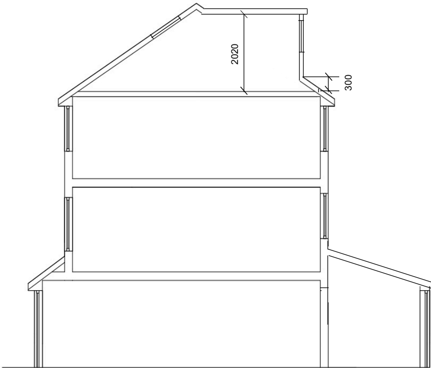
Proposed Elevations
