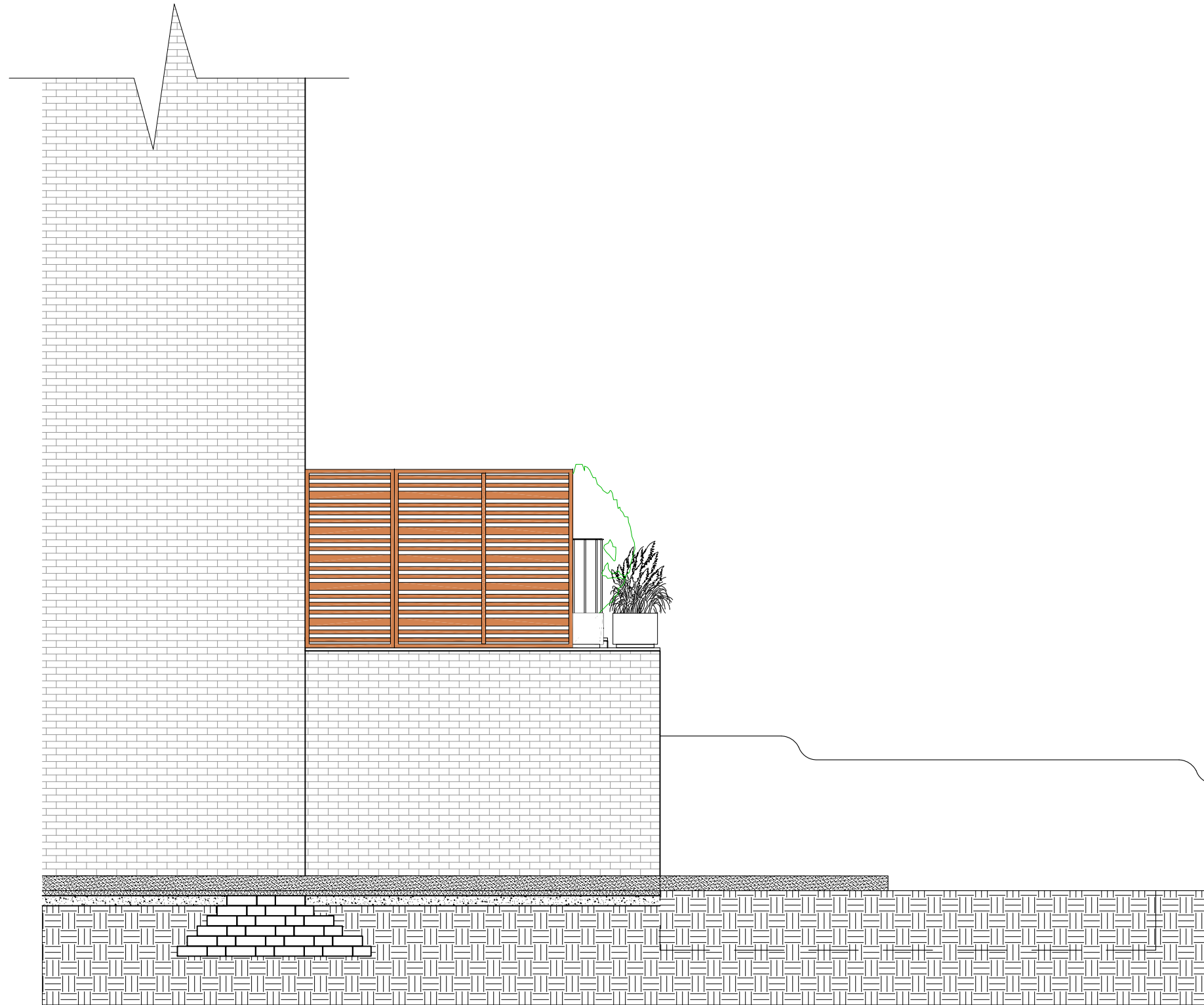
1 LEVEL B01 - EXISTING ELEVATION WEST SCALE : 1:50 @ A3
