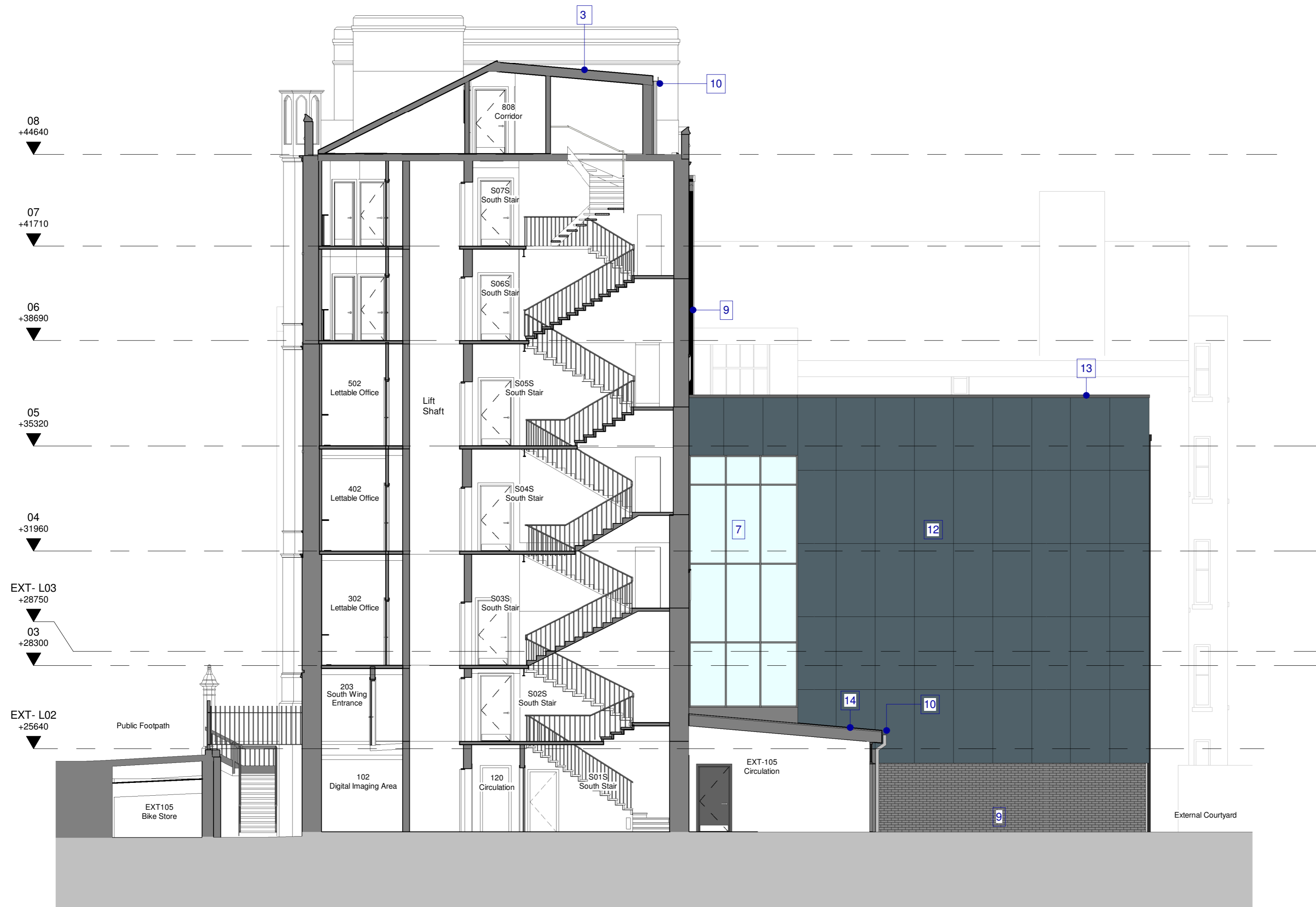
Proposed Elevations - Elevation A 1 : 100
