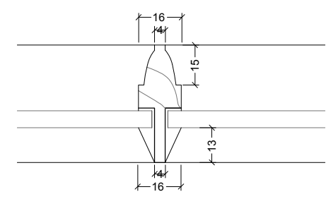
06 DOOR TYPE 2D - GLAZING BAR 1:2@A3, 1:1@A1
