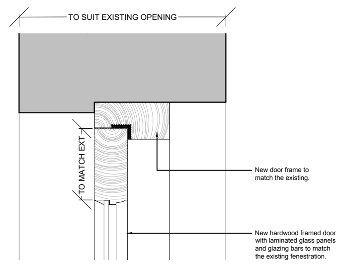
03 DOOR TYPE 2D - HEAD DETAIL 1:5@A3, 1:2.5@A1
