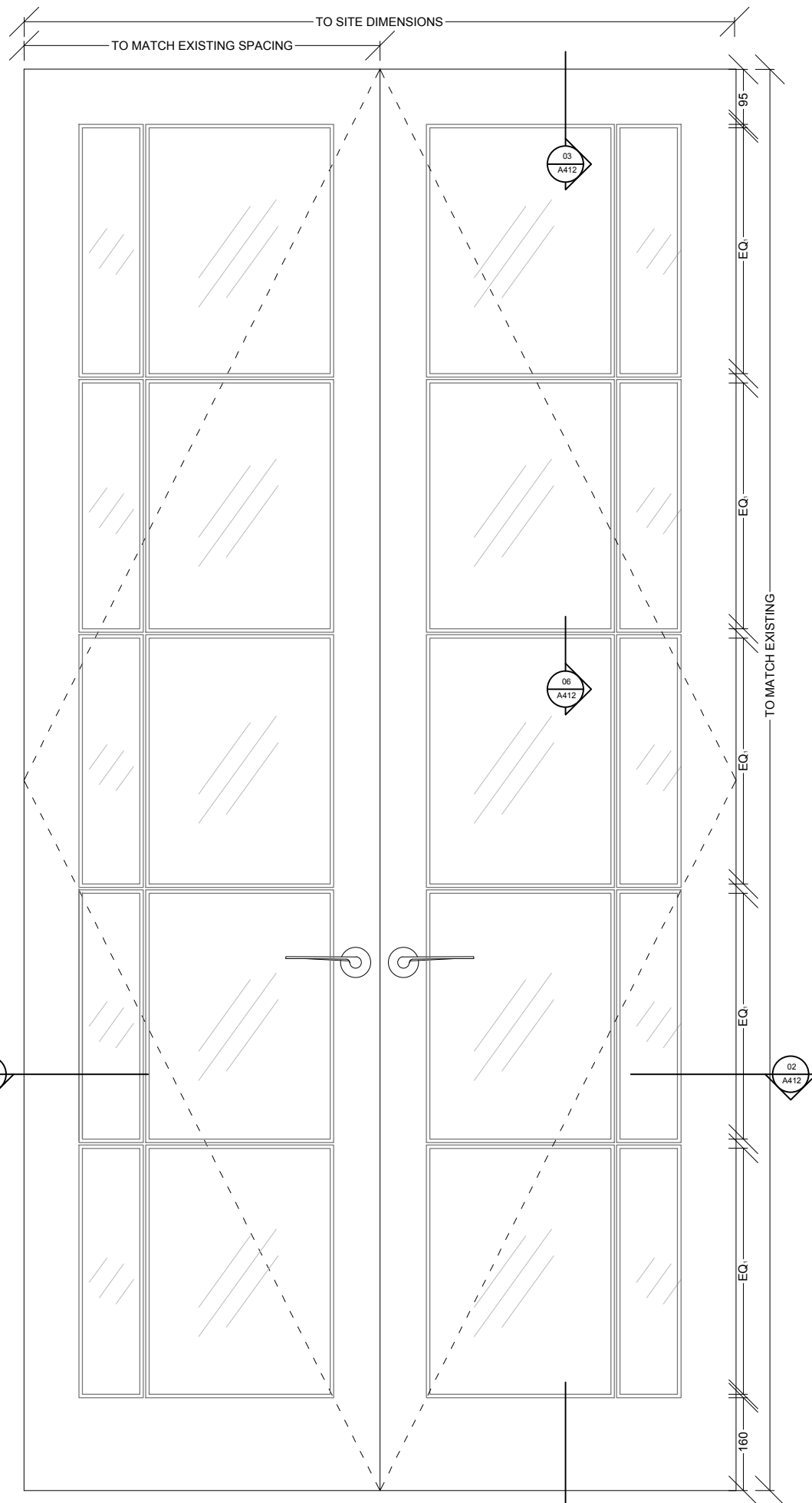
01 DOOR TYPE 2D - PROPOSED ELEVATION 1:20@A3, 1:10@A1
