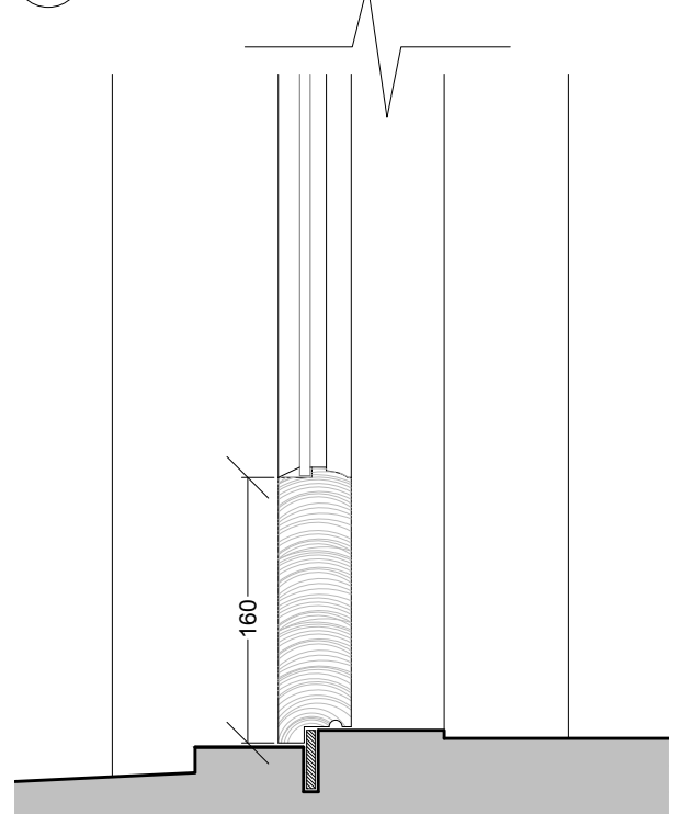
04 DOOR TYPE 2D - THRESHOLD DETAIL 1:5@A3, 1:2.5@A1
