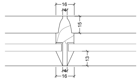
06 DOOR TYPE 2D - GLAZING BAR 1:2@A3, 1:1@A1
