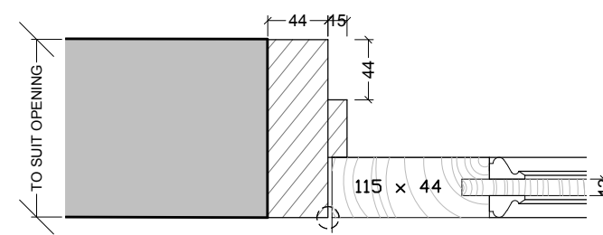
05 DOOR TYPE 1A - JAMB DETAIL 1:5@A3, 1:2.5@A1
