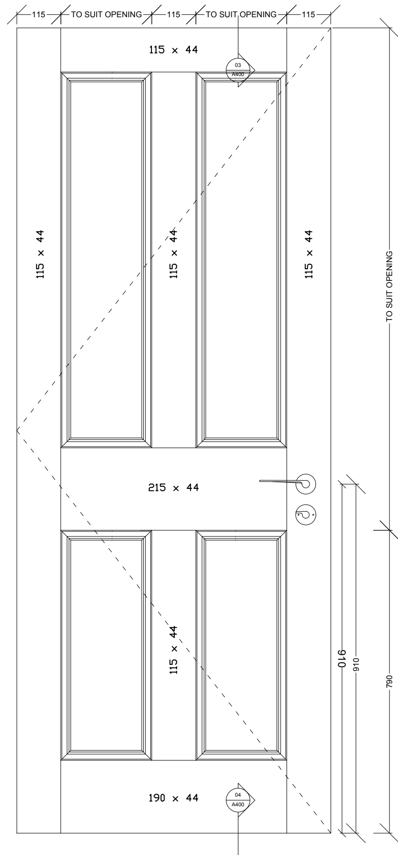
01 DOOR TYPE 1A - PROPOSED ELEVATION 1:10@A3, 1:5@A1
