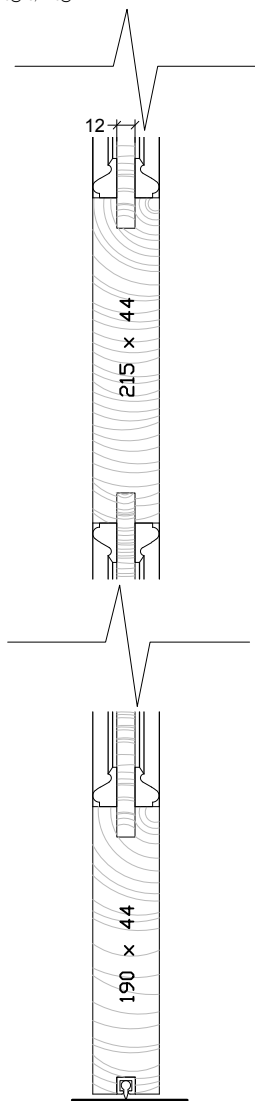
04 DOOR TYPE 1A - THRESHOLD DETAIL 1:5@A3, 1:2.5@A1
