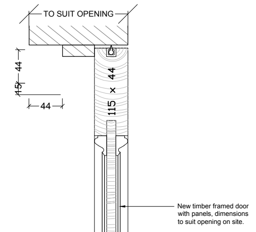
03 DOOR TYPE 1A - HEAD DETAIL 1:5@A3, 1:2.5@A1
