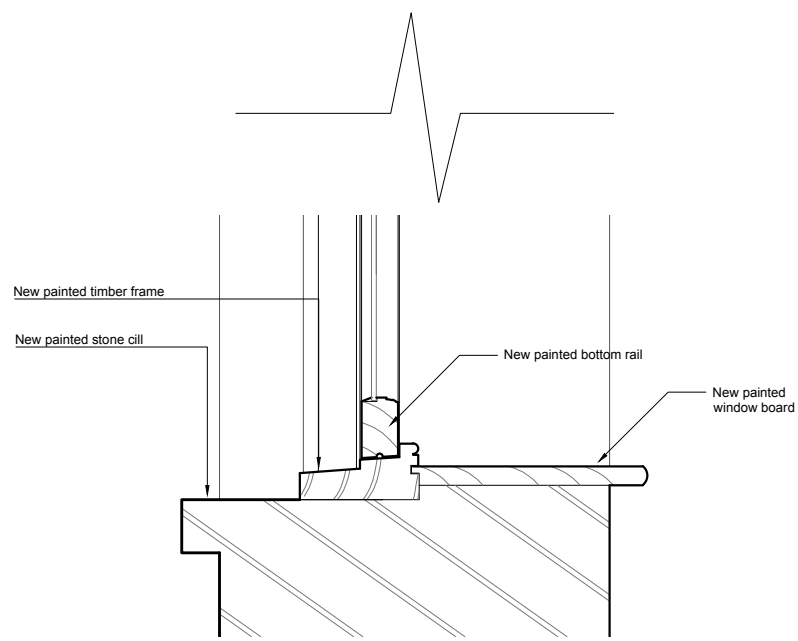
05 WINDOW TYPE 2C - CILL 1:10@A3, 1:5@A1
