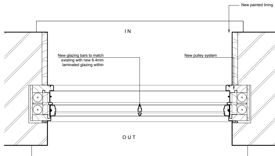
02 WINDOW TYPE 2B - JAMBS 1:10@A3,1:5@A1
