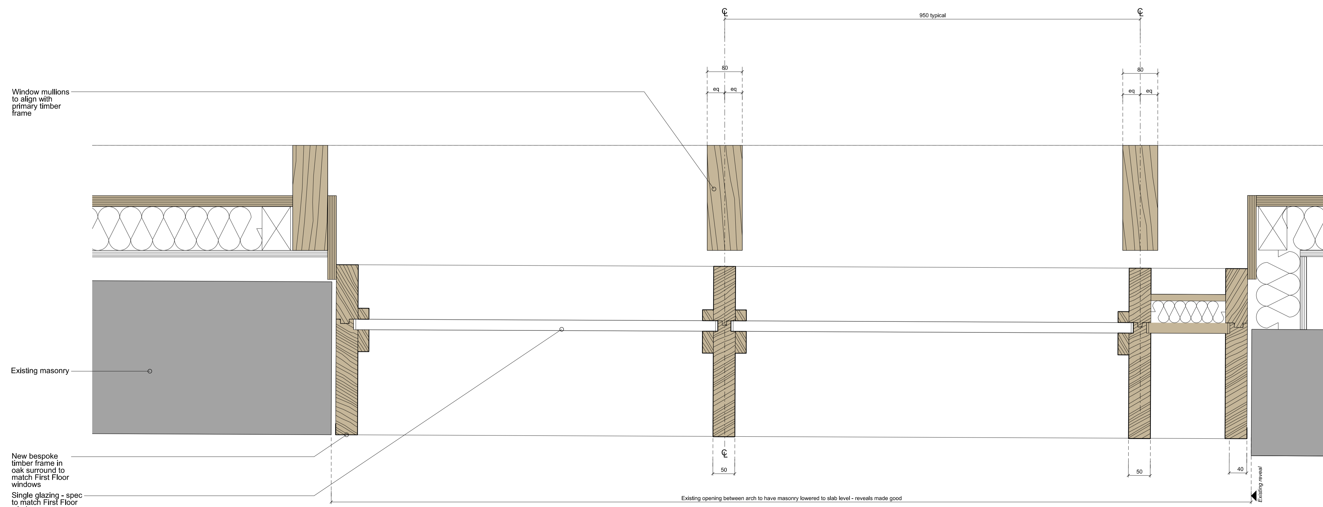
01 Proposed Plan detail showing Ground Floor window 7D(PL)28 7 Denmark Street - Mews 1:5
