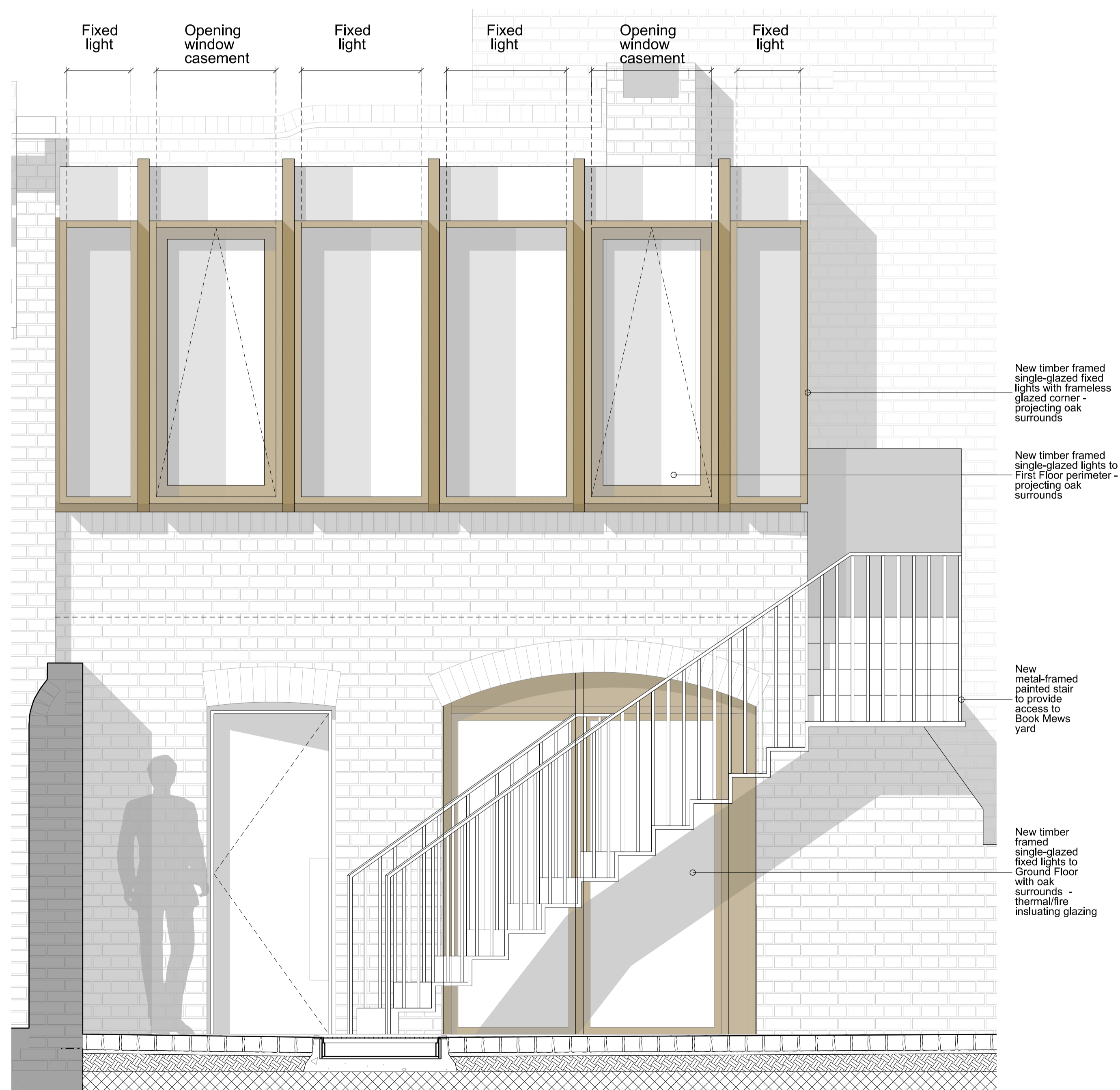
01 Proposed Detailed Elevation - facing yard 7D(PL)25 7 Denmark Street - Mews 1:20
