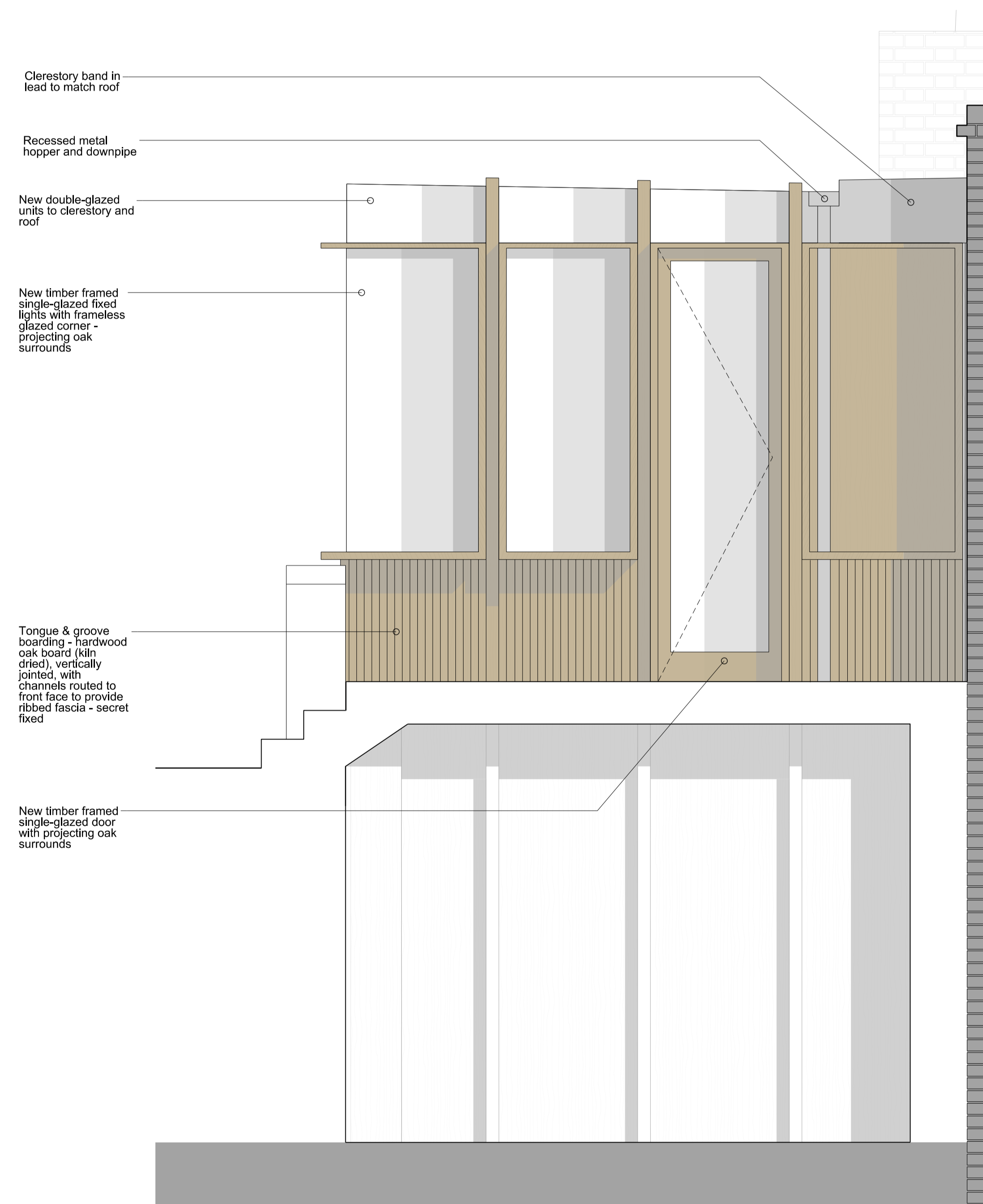
02 Proposed Detailed Elevation - facing no. 8 Denmark Street 7D(PL)25 7 Denmark Street - Mews 1:20
