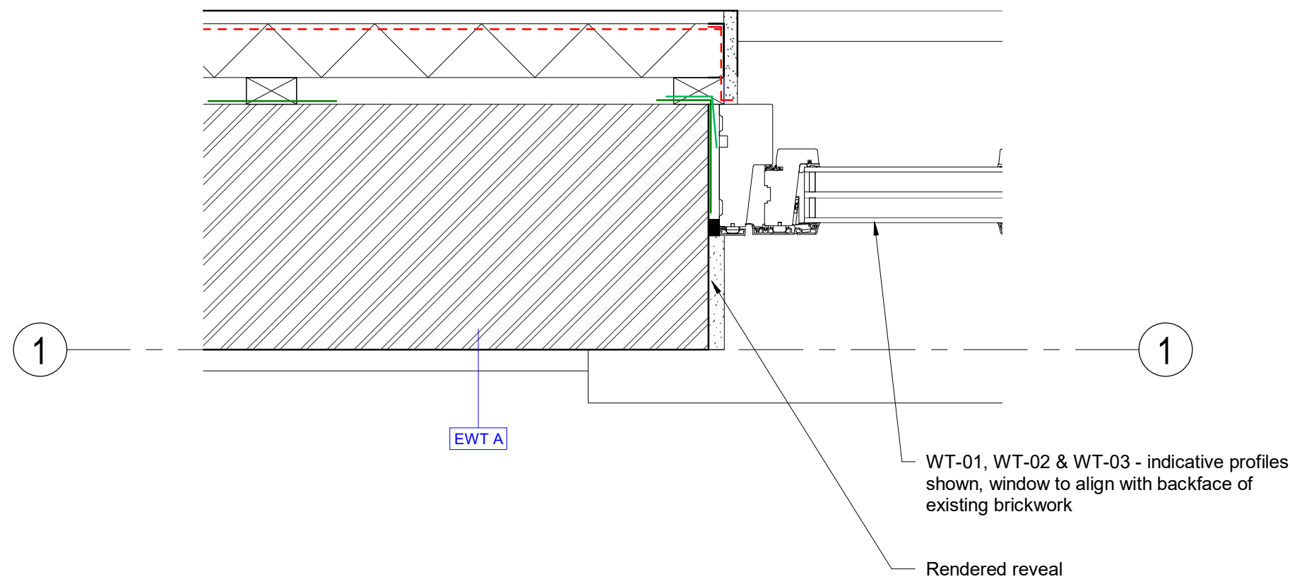
2 EWTA - Typical Window jamb detail - WT-01,02,03 3201 1 : 5
