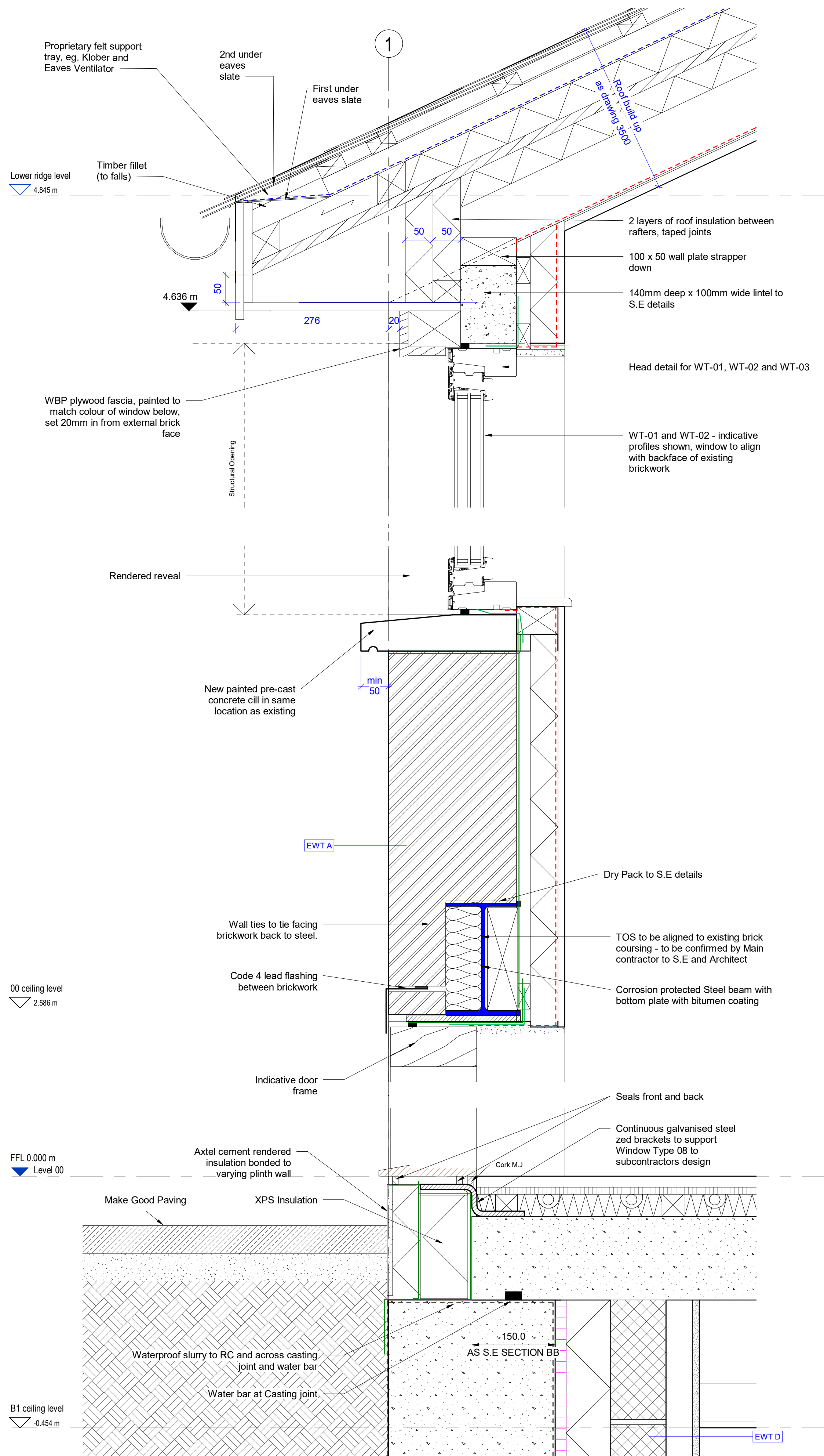
1 EWTA - Window openings and roof details 3201 1 : 5
