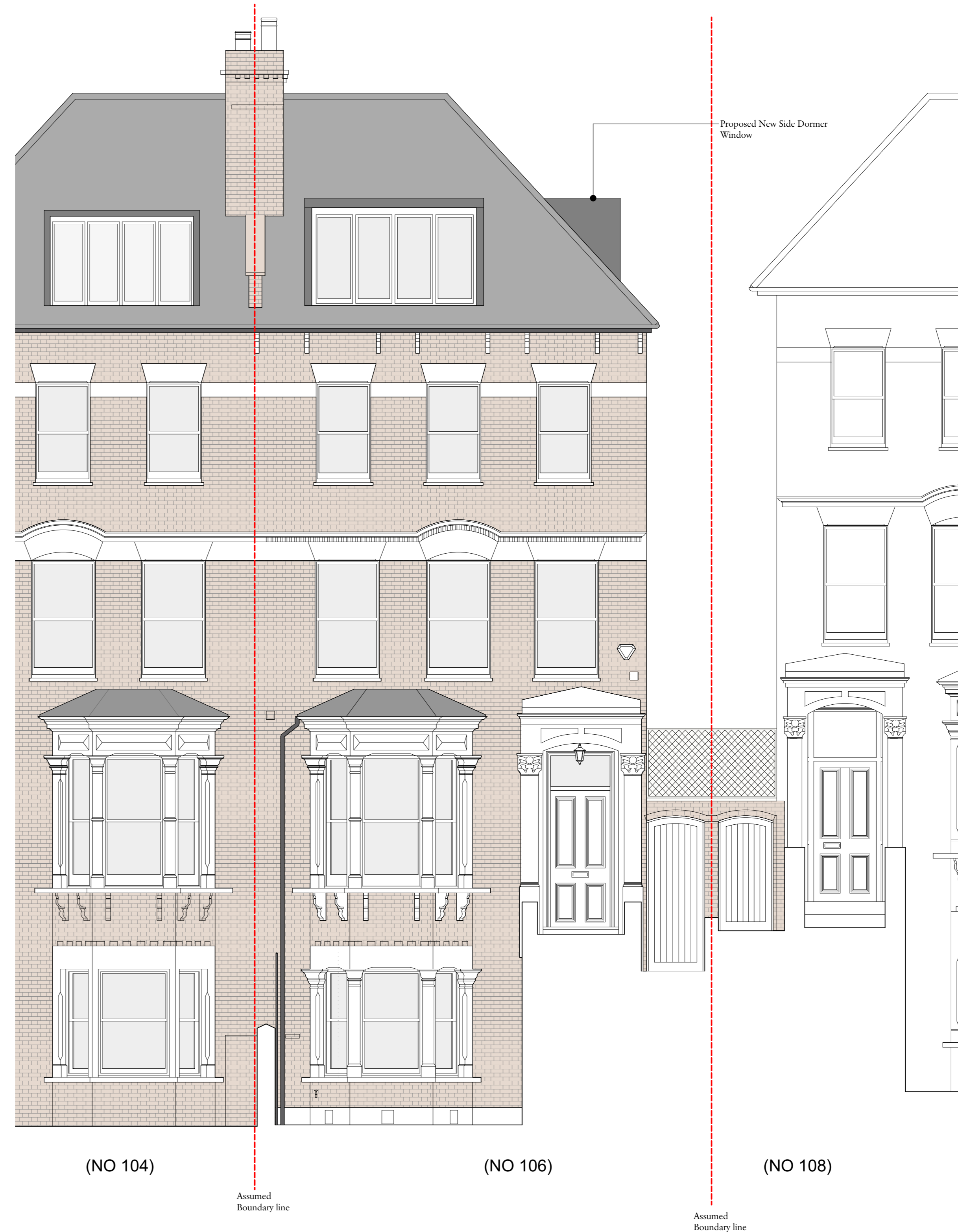
2 Proposed South East Elevation
