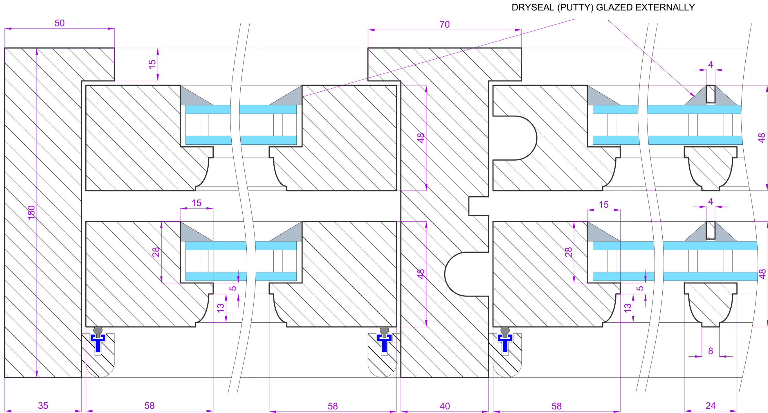
SECTION THROUGH FRAME JAMB, MULLION AND GLAZING BAR SCALE 1:1 ON A3
