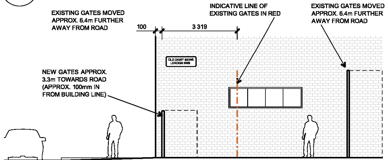
5 PROPOSED SECTION A 001 1:100 @ A3
