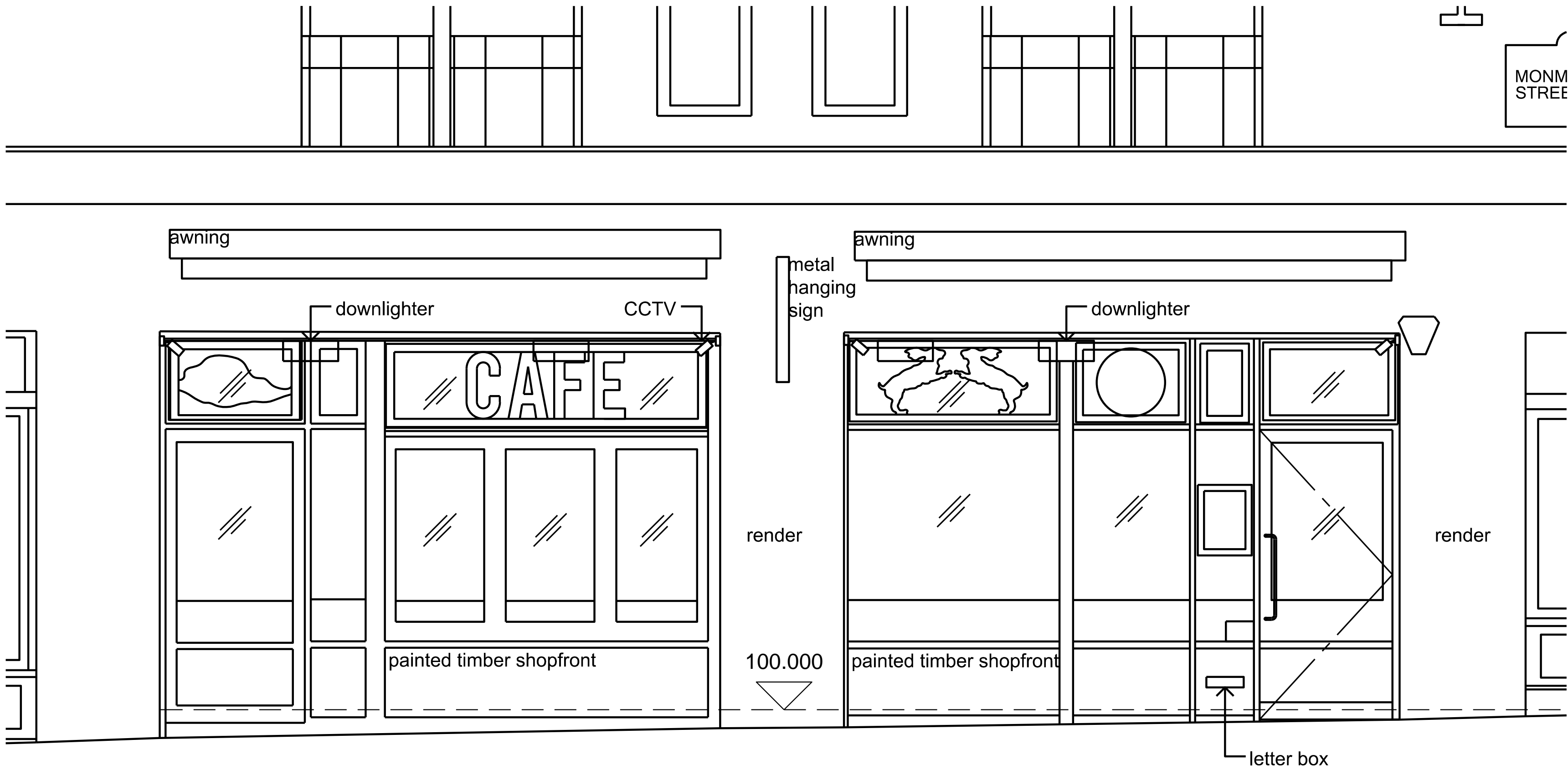
Existing Shopfront
