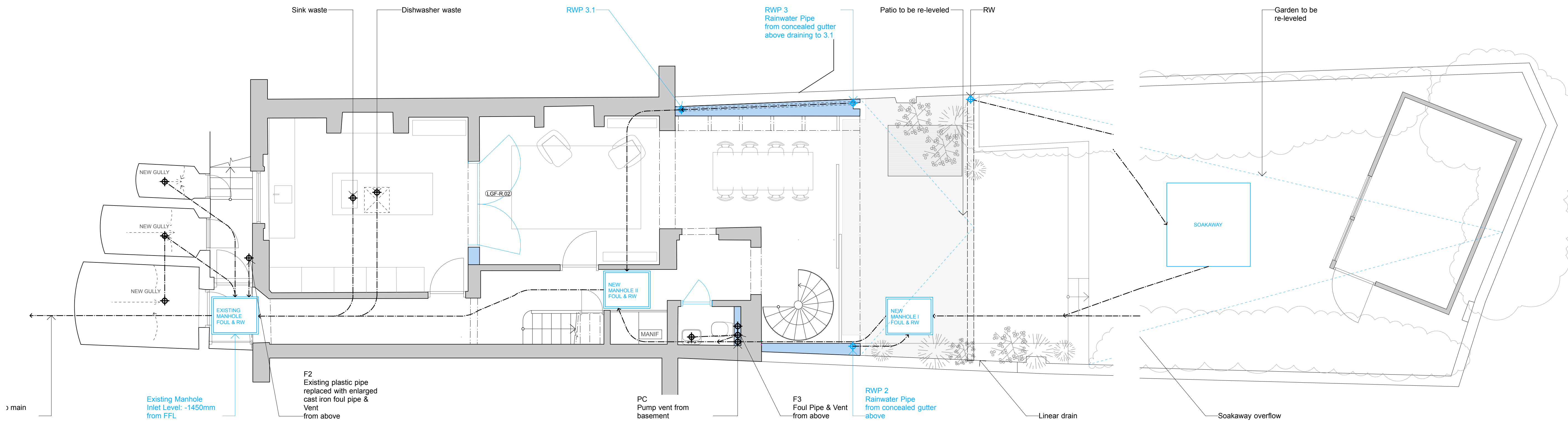
2 BELOW GROUND DRAINAGE - LOWER GROUND FLOOR 1:50
