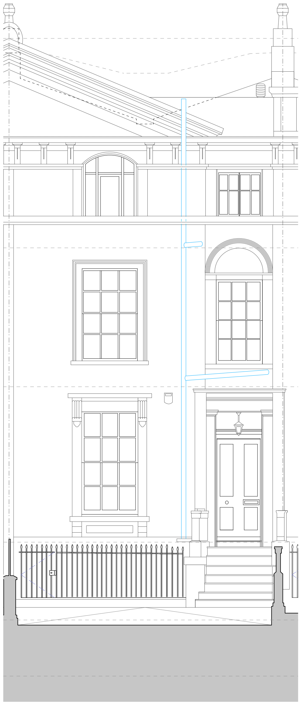
4 DRAINAGE - FRONT ELEVATION 1:50 @ A1
