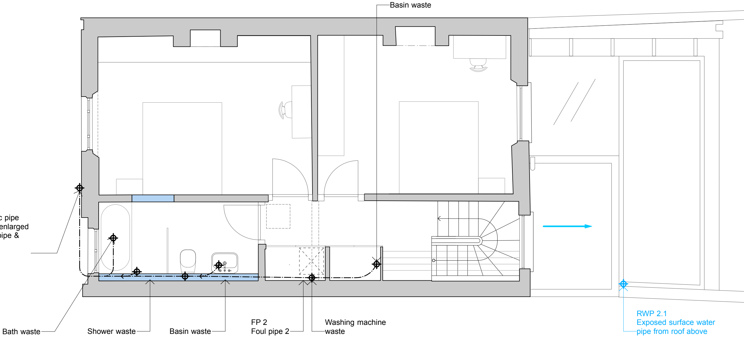
1 DRAINAGE - SECOND FLOOR 1:50 @ A1
