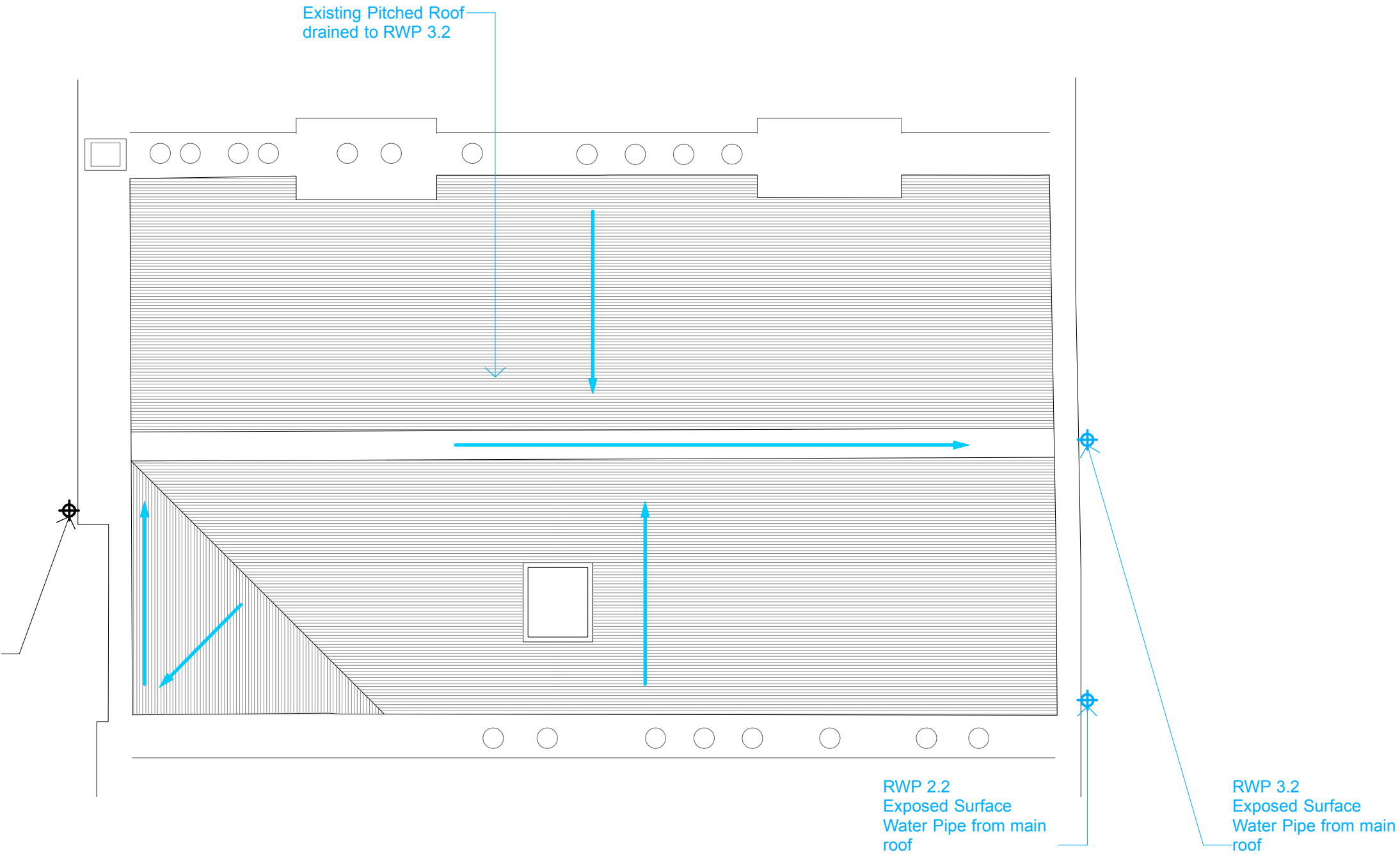
2 DRAINAGE - ROOF TOP VIEW 1:50 @ A1
