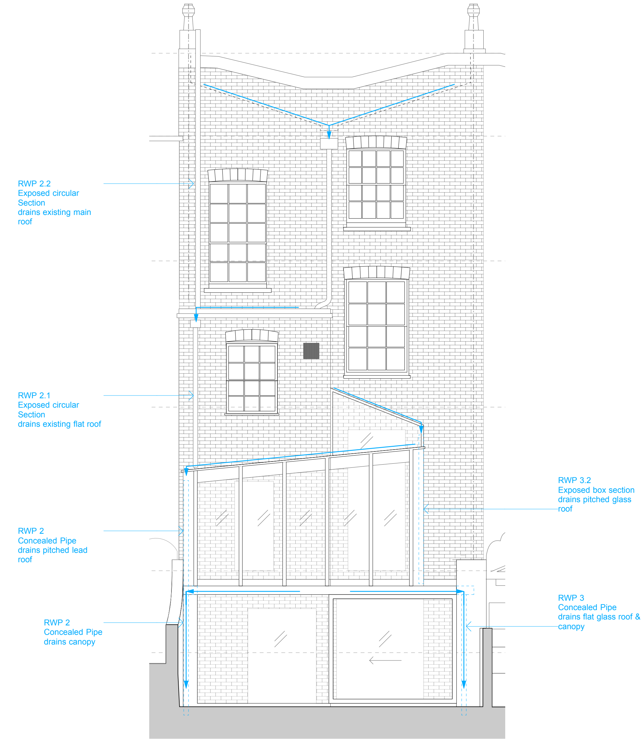
3 DRAINAGE - REAR ELEVATION 1:50 @ A1
