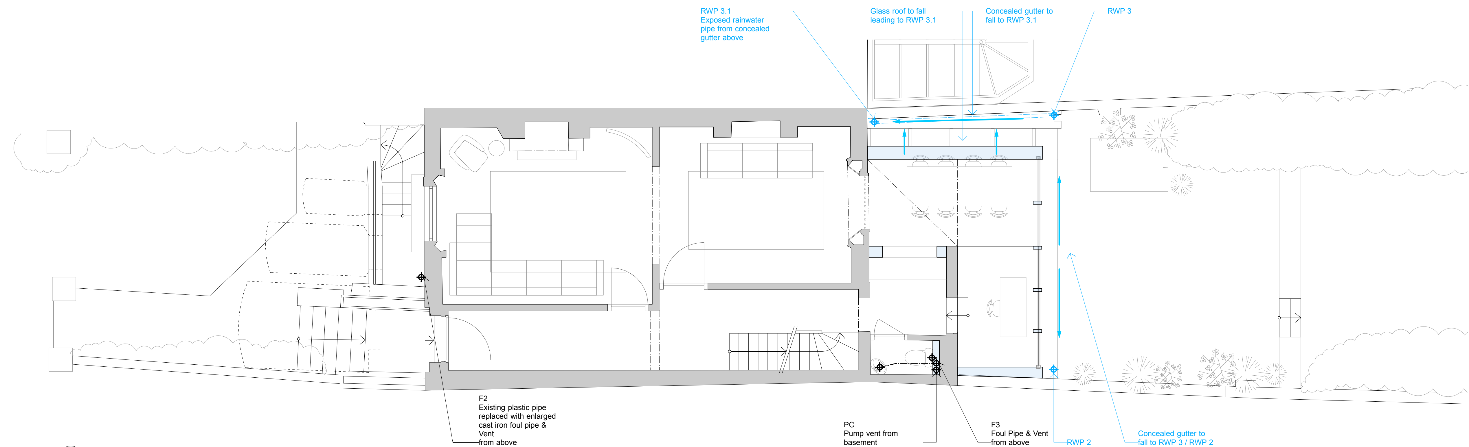
1 DRAINAGE - GROUND FLOOR 1:50 @ A1
