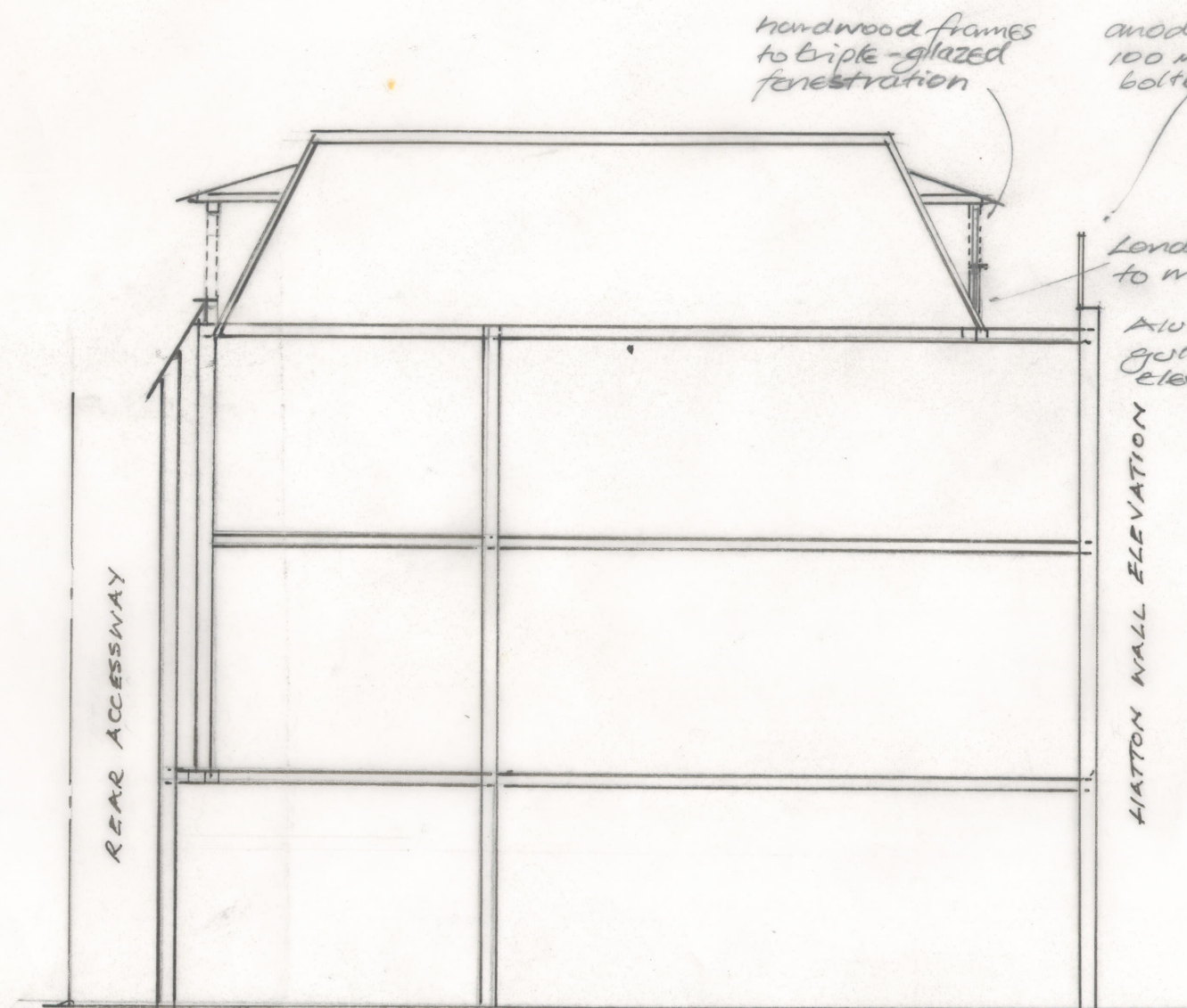
PROPOSED SECTION FACING N.E.
