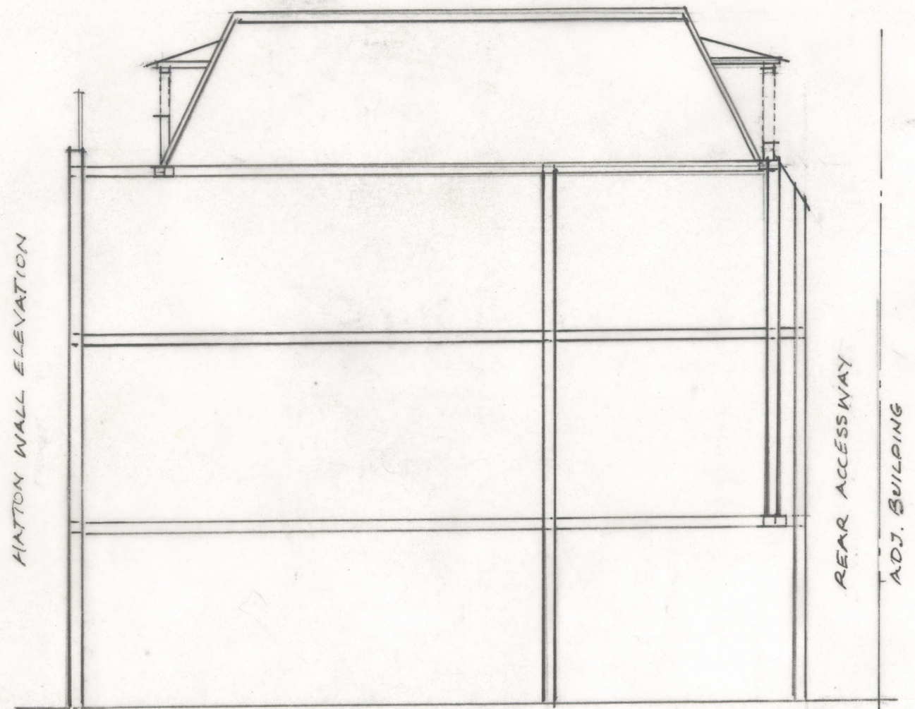
PROPOSED SECTION FACING S.W.
