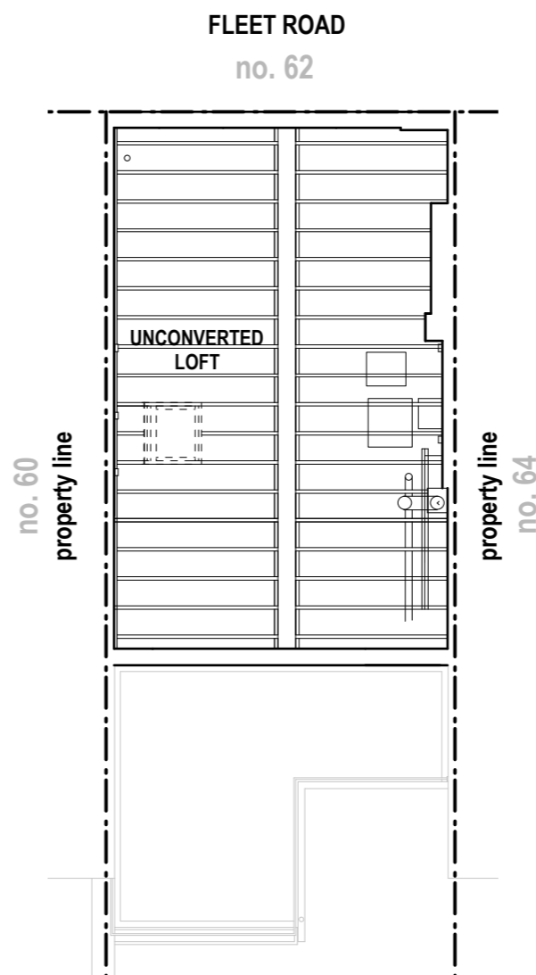
Existing Loft / Roof Structure Plan
