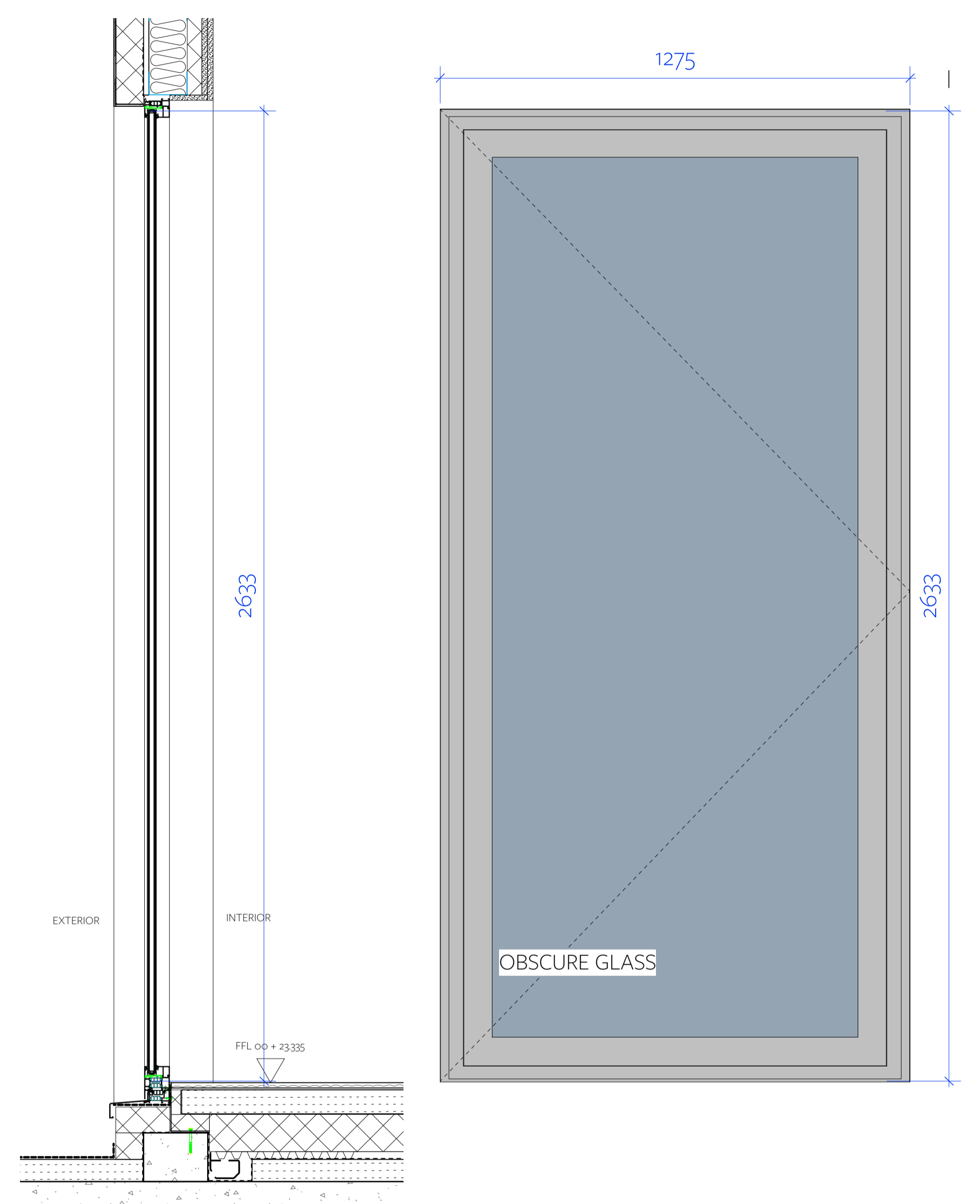
Section
