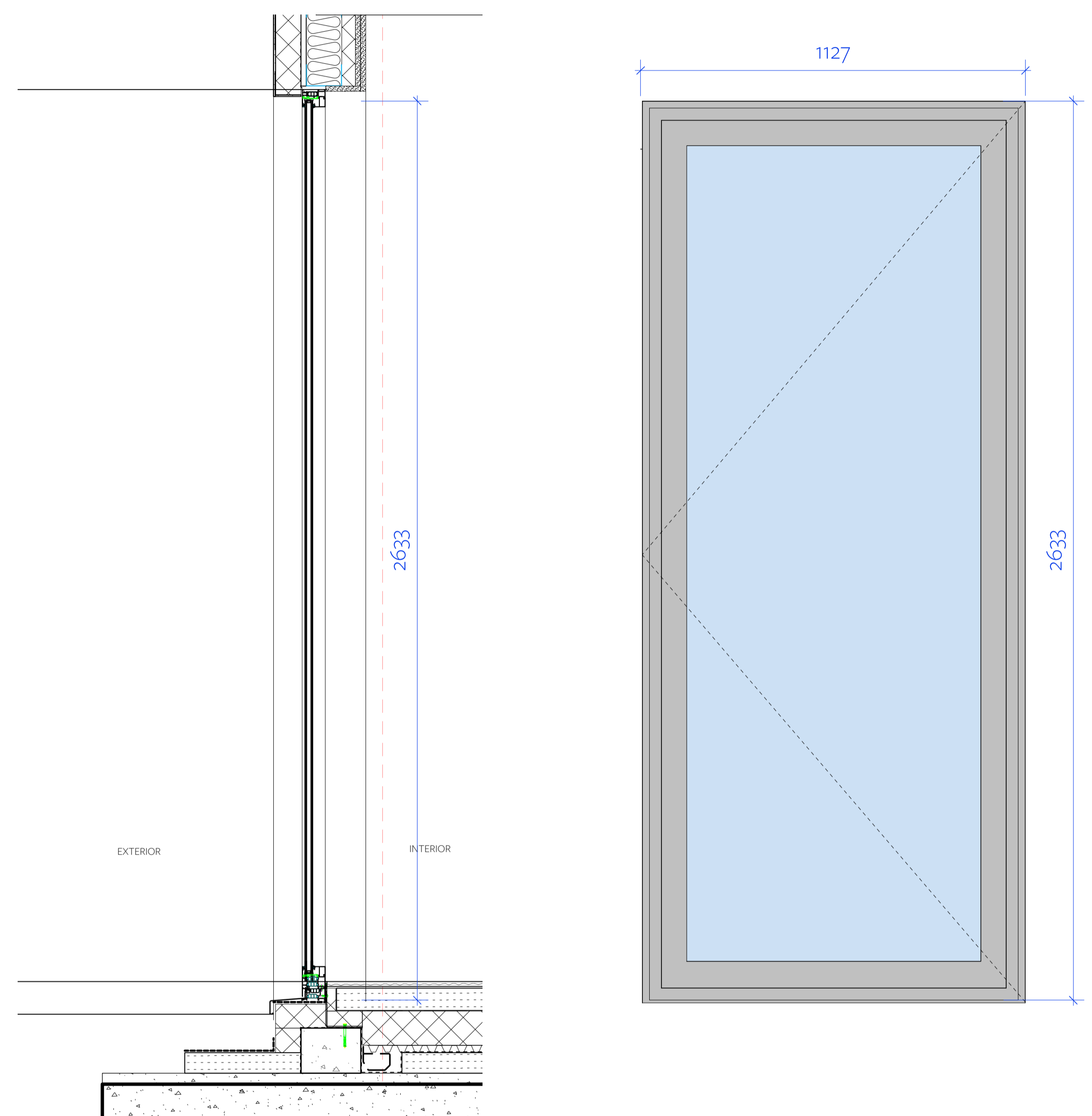
Section
