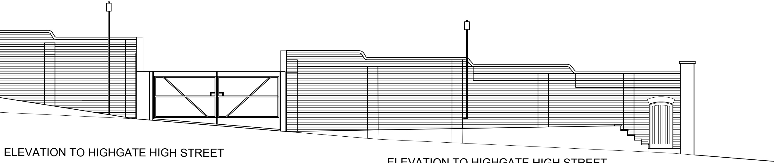
ELEVATION TO HIGHGATE HIGH STREET
