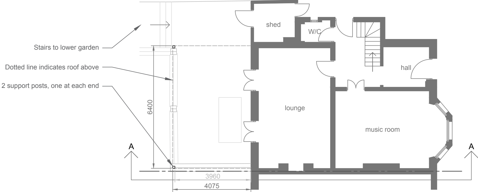
Floor Plan
