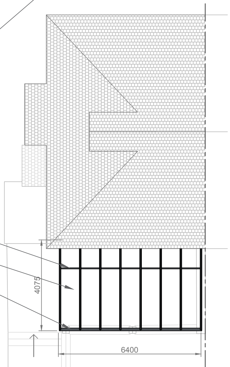
Roof Plan
