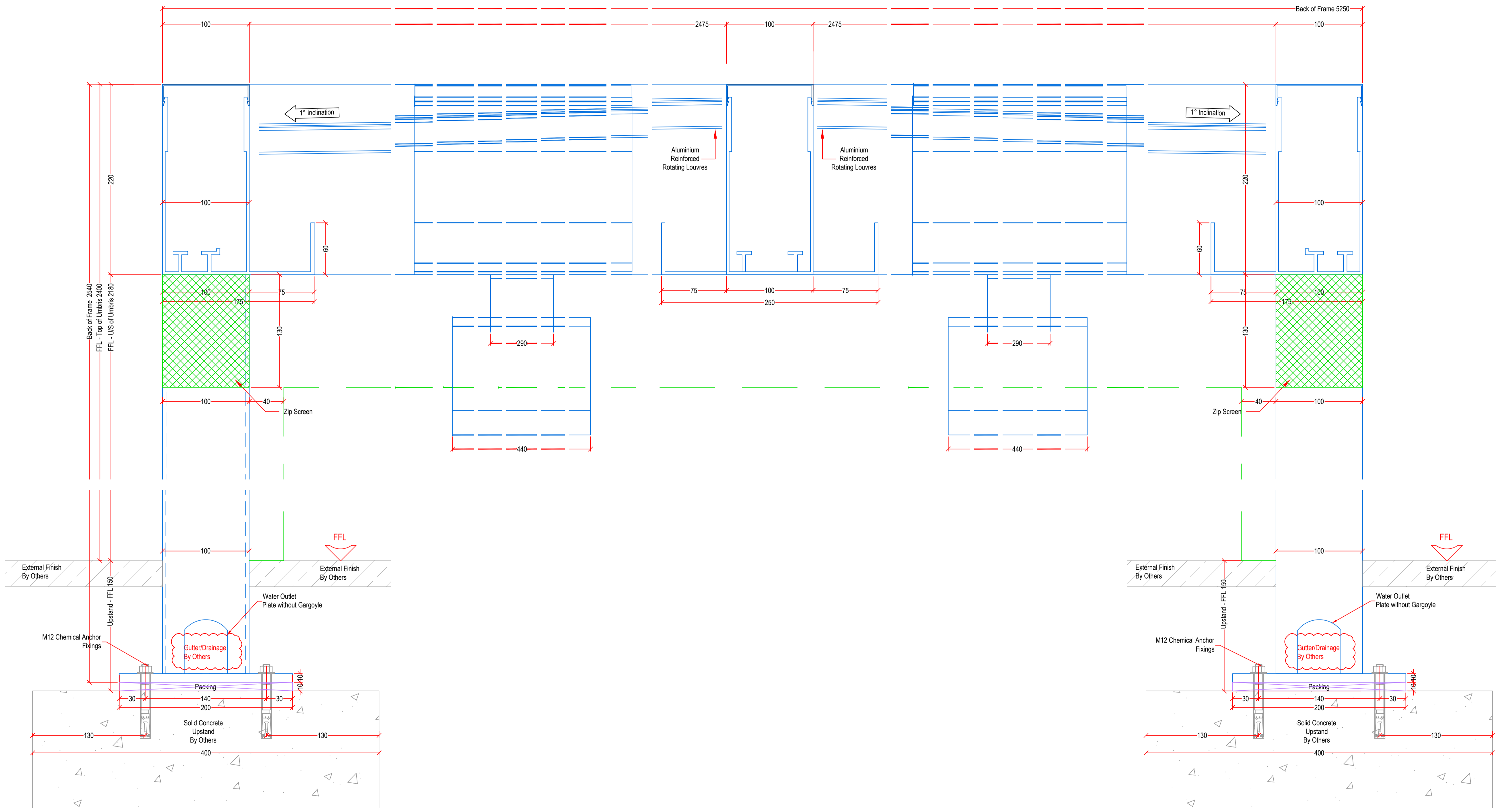
Umbris Automated Louvre System - Section A-A Scale 1:2.5
