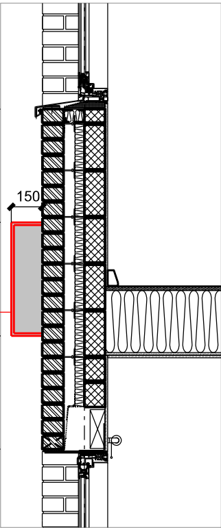
2 Signage detail 1:20
