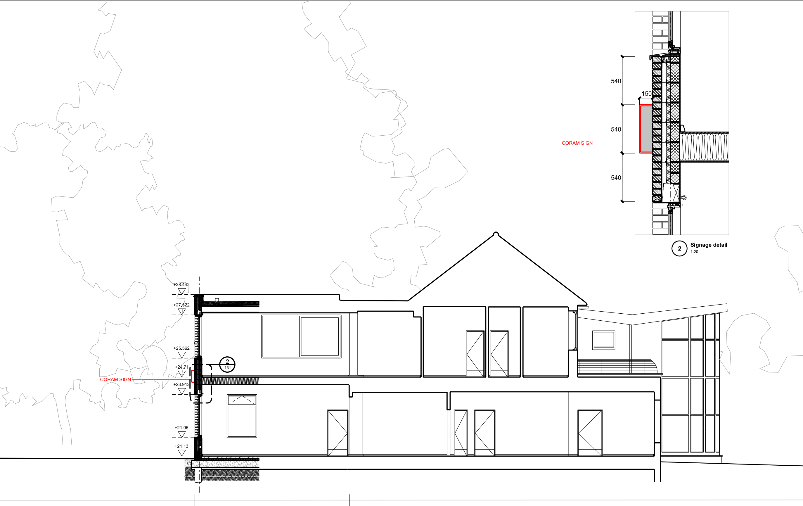
1 Existing Section EE 1:100
