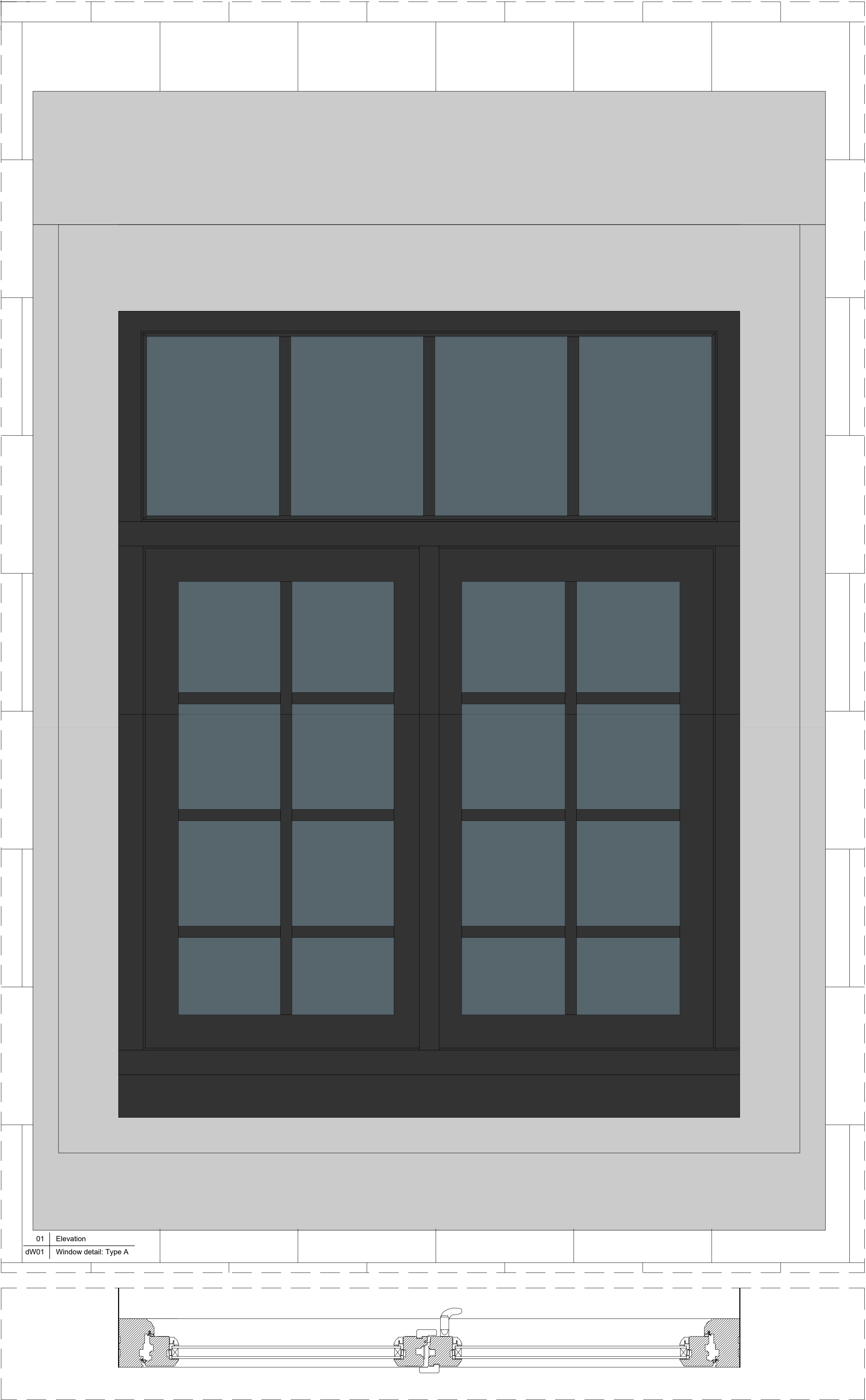
02 Plan dW01 Window detail: Type A
