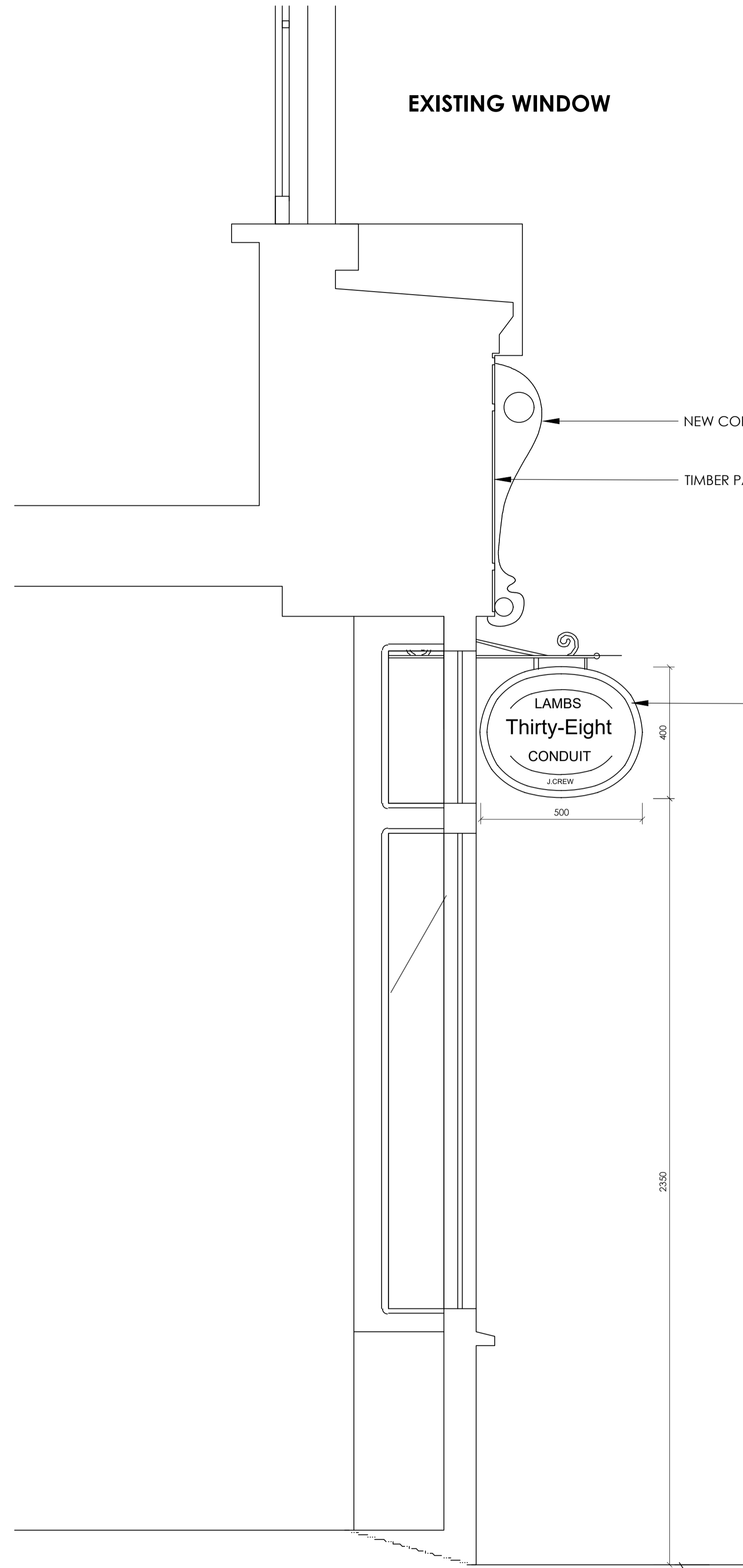
6 PROPOSED SHOPFRONT SECTION 1:10 @ A1 - 1:20 @ A3
