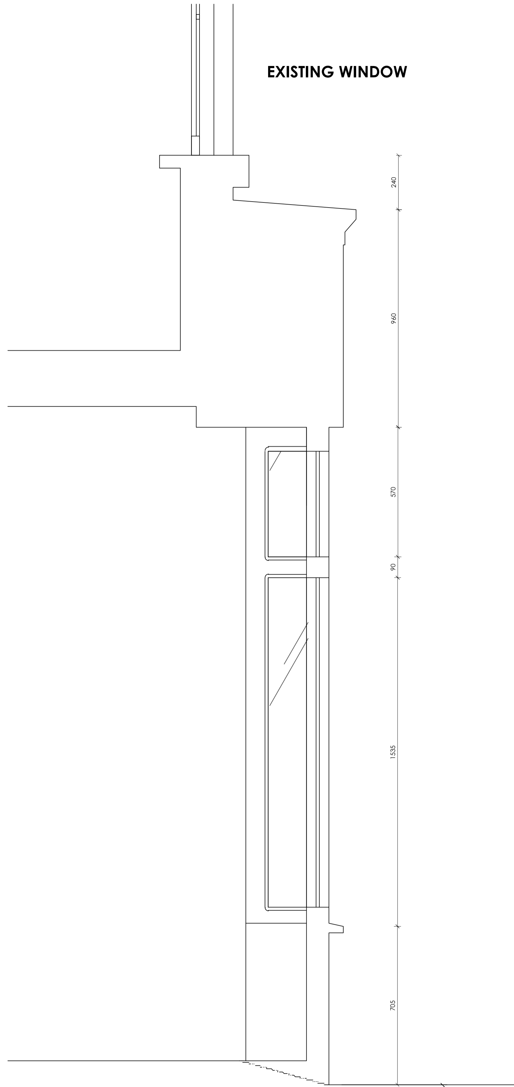
5 EXISTING SHOPFRONT SECTION 1:10 @ A1 - 1:20 @ A3
