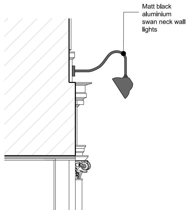
Lighting side elevation
