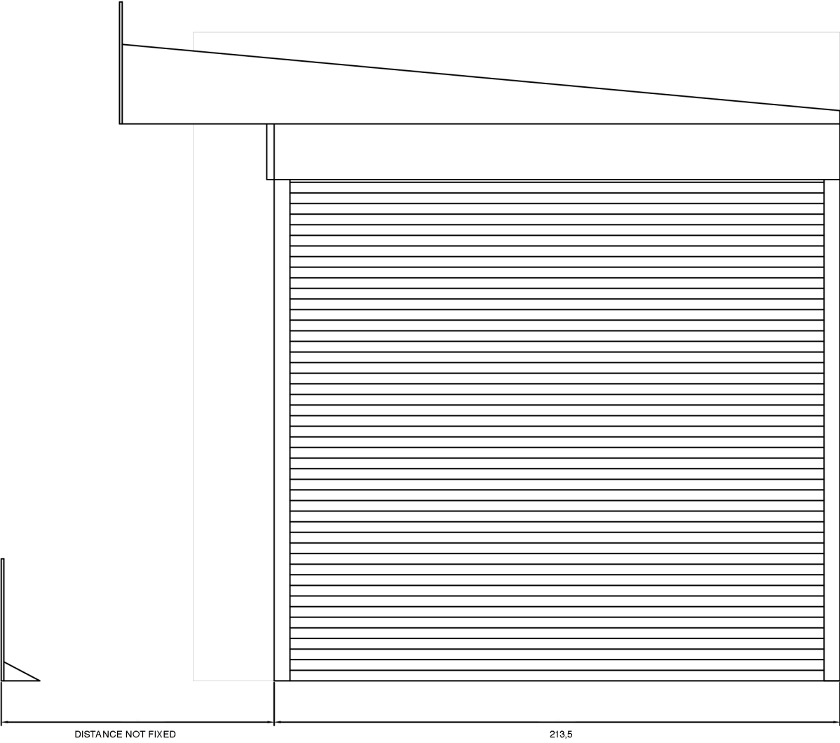
EAST ELEVATION
