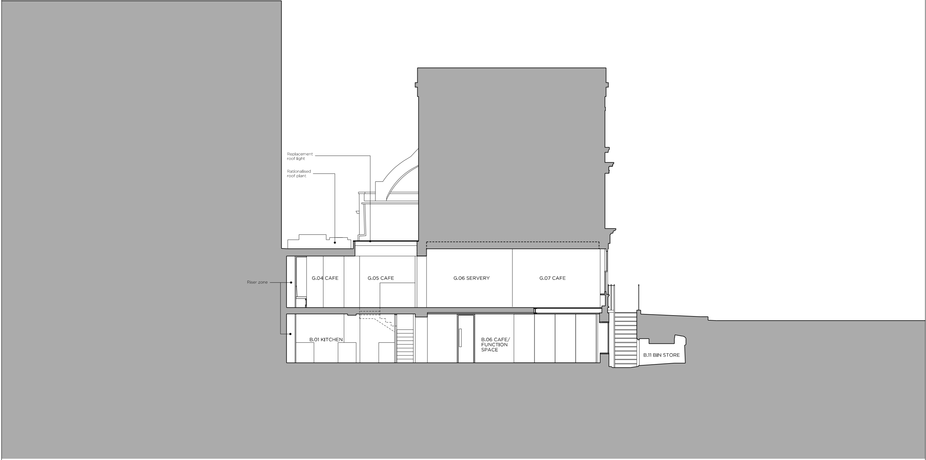
01 LONG SECTION
